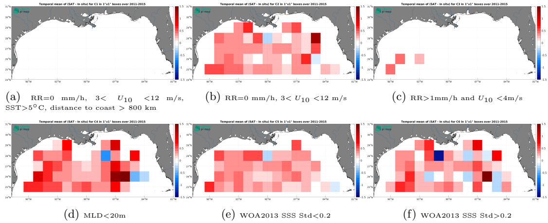
Figure 14: Temporal mean gridded over spatial boxes of size 1^\circ \times 1^\circ of \Delta SSS (Aquarius SSS L3 CAP v5 - 7-Day running (JPL) - Argo) for 6 different subdatasets corresponding to:RR=0 mm/h, 3 < U_{10} < 12 m/s, SST >5^\circ\text{C} , distance to coast > 800 km (a), RR=0 mm/h, 3 < U_{10} < 12 m/s (b), RR >1 mm/h and U_{10} < 4 m/s (c),MLD <20 m (d),WOA2013 SSS Std <0.2 (e),WOA2013 SSS Std >0.2 (f).
