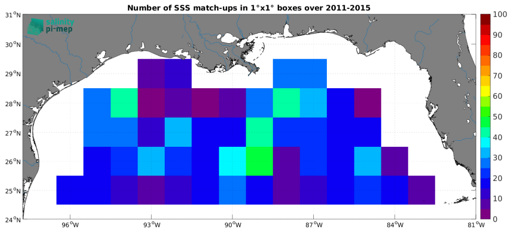
Figure 5: Number of SSS match-ups between Argo SSS and the Aquarius SSS L3 CAP v5 - 7-Day running (JPL) SSS product for the Mississippi river plume Pi-MEP region over 1^\circ \times 1^\circ boxes and for the full satellite product period.
