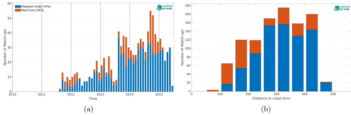
Figure 2: Number of match-ups between Argo and Aquarius SSS L3 CAP v5 - 7-Day running (JPL) SSS as a function of time (a) and as function of the distance to coast (b) over the Mississippi river plume Pi-MEP region and for the full satellite product period.
