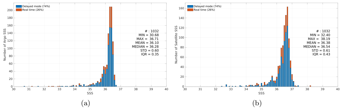
Figure 3: Histograms of SSS from Argo (a) and Aquarius SSS L3 CAP v5 - 7-Day running (JPL) (b) considering all match-up pairs per bins of 0.1 over the Mississippi river plume Pi-MEP region and for the full satellite product period.
