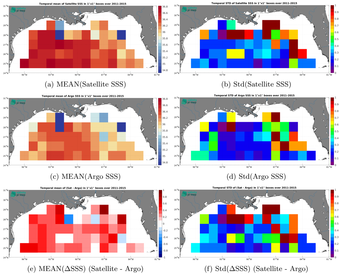
Figure 7: Temporal mean (left) and Std (right) of SSS from Aquarius SSS L3 CAP v5 - 7-Day running (JPL) (top), Argo (middle), and of \Delta SSS (Satellite - Argo). Only match-up pairs are used to generate these maps.
