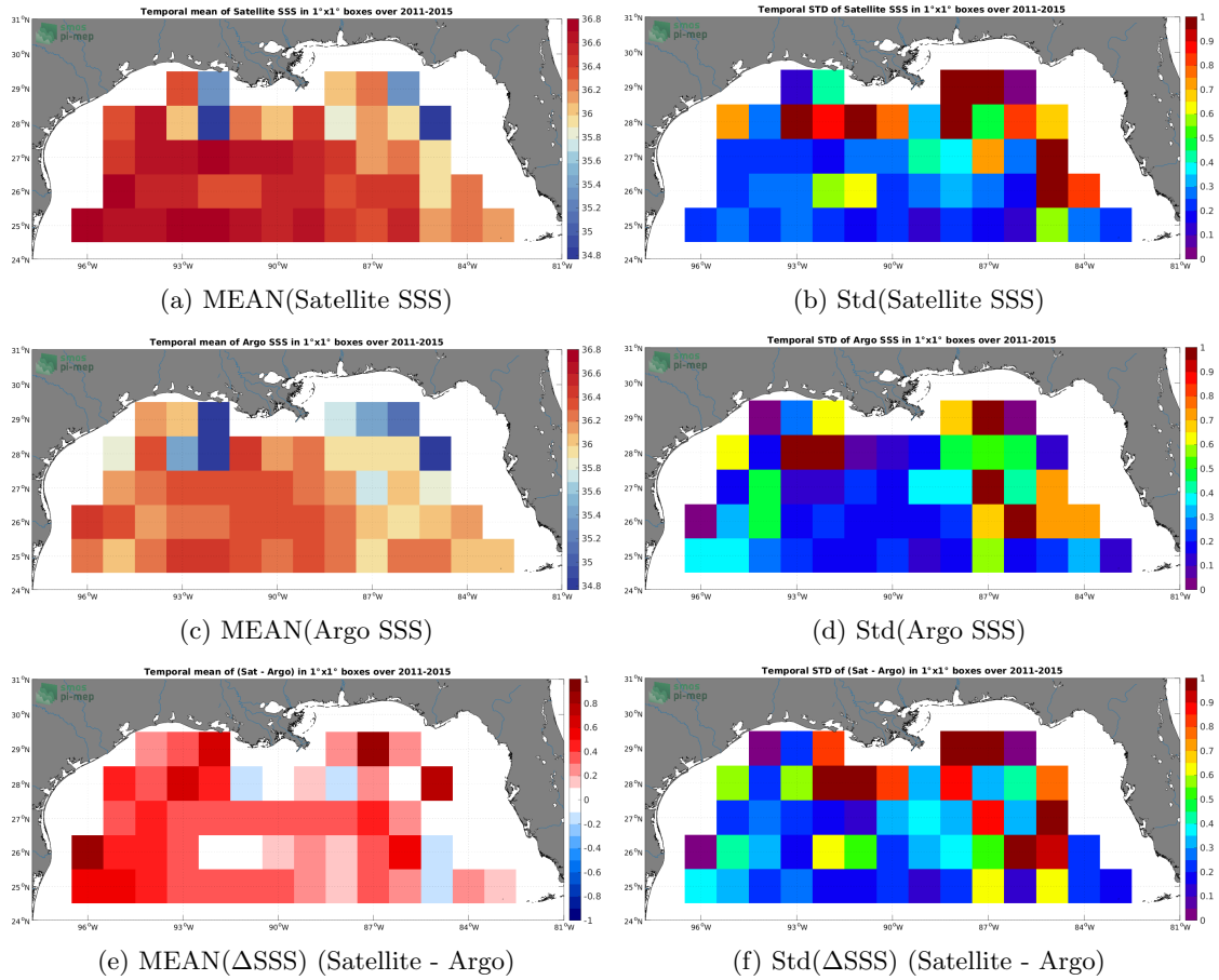
Figure 6: Temporal mean (left) and Std (right) of SSS from Aquarius SSS L3 CAP v5 - 7-Day running (JPL) (top), Argo (middle), and of \Delta SSS (Satellite - Argo). Only match-up pairs are used to generate these maps.
