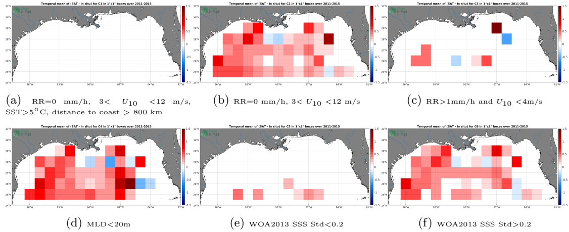
Figure 12: Temporal mean gridded over spatial boxes of size 1^{\circ} \times 1^{\circ} of \Delta\text{SSS} (Aquarius SSS L3 CAP v5 - 7-Day running (JPL) - Argo) for 6 different subdatasets corresponding to: \text{RR}=0 mm/h, 3 < U_{10} < 12 m/s, \text{SST} > 5^{\circ}\text{C} , distance to coast > 800 km (a), \text{RR}=0 mm/h, 3 < U_{10} < 12 m/s (b), \text{RR} > 1\text{mm/h} and U_{10} < 4\text{m/s} (c), \text{MLD} < 20\text{m} (d), \text{WOA2013 SSS Std} < 0.2 (e), \text{WOA2013 SSS Std} > 0.2 (f).
