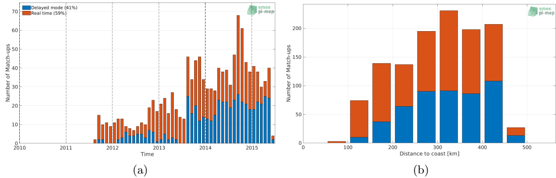
Figure 1: Number of match-ups between Argo and Aquarius SSS L3 CAP v5 - 7-Day running (JPL) SSS as a function of time (a) and as function of the distance to coast (b) over the Mississippi river plume Pi-MEP region and for the full satellite product period.
