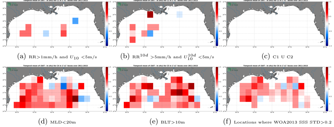
Figure 12: Temporal mean gridded over spatial boxes of size 1^\circ \times 1^\circ of \Delta\text{SSS} (Aquarius-L3-JPL-V5-7DAY-RUNNING - Argo) for 6 different subdatasets corresponding to: \text{RR} > 1\text{mm/h} and U_{10} < 5\text{m/s} (a), \text{RR}^{10d} > 5\text{mm/h} and U_{10}^{10d} < 5\text{m/s} (b), C1 U C2 (c), \text{MLD} < 20\text{m} (d), \text{BLT} > 10\text{m} (e), Locations where WOA2013 SSS STD > 0.2 (f).
