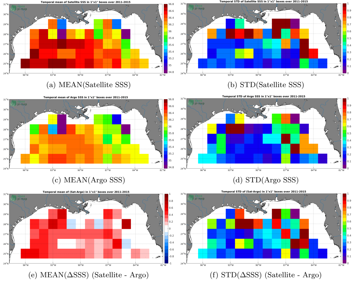
Figure 6: Temporal mean (left) and STD (right) of SSS from Aquarius-L3-JPL-V5-7DAY-RUNNING (top), Argo (middle), and of \Delta SSS (Satellite - Argo). Only match-up pairs are used to generate these maps.
