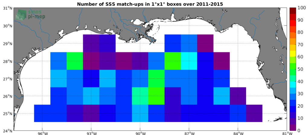
Figure 4: Number of SSS match-ups between Argo SSS and the Aquarius-L3-JPL-V5-7DAY-RUNNING SSS product for the Mississippi river plume Pi-MEP region over 1^\circ \times 1^\circ boxes and for the full satellite product period.
