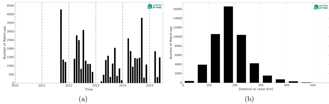
Figure 2: Number of match-ups between TSG (SAMOS) and Aquarius SSS L3 CAP v5 - Monthly (JPL) SSS as a function of time (a) and as function of the distance to coast (b) over the Mississippi river plume Pi-MEP region and for the full satellite product period.
