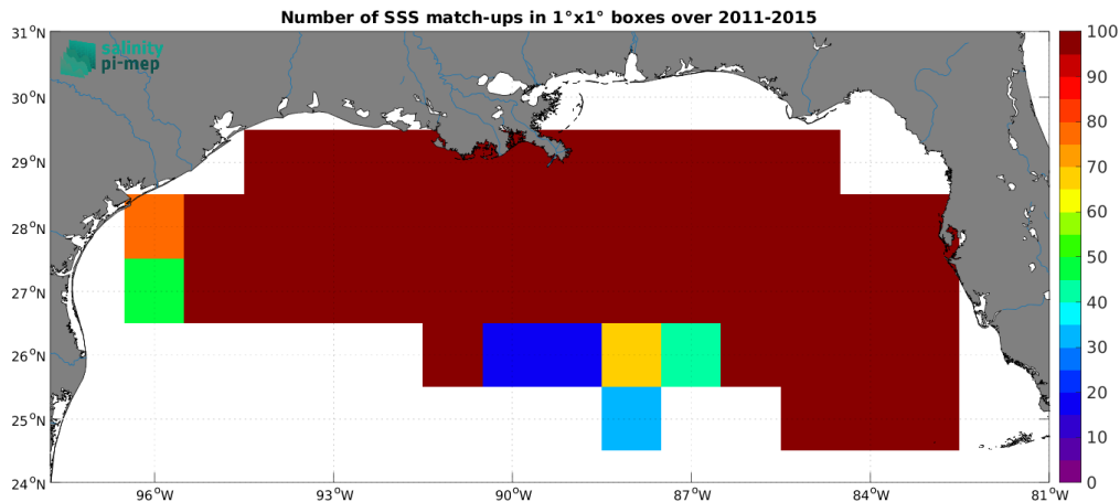
Figure 5: Number of SSS match-ups between TSG (SAMOS) SSS and the Aquarius SSS L3 CAP v5 - Monthly (JPL) SSS product for the Mississippi river plume Pi-MEP region over 1^\circ \times 1^\circ boxes and for the full satellite product period.
