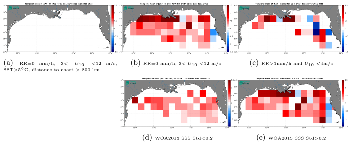
Figure 14: Temporal mean gridded over spatial boxes of size 1^\circ \times 1^\circ of \Delta SSS (Aquarius SSS L3 CAP v5 - Monthly (JPL) - TSG (SAMOS)) for 5 different subdatasets corresponding to:RR=0 mm/h, 3 < U_{10} < 12 m/s, SST > 5^\circ C , distance to coast > 800 km (a), RR=0 mm/h, 3 < U_{10} < 12 m/s (b), RR>1mm/h and U_{10} < 4 m/s (c), WOA2013 SSS Std<0.2 (d), WOA2013 SSS Std>0.2 (e).
