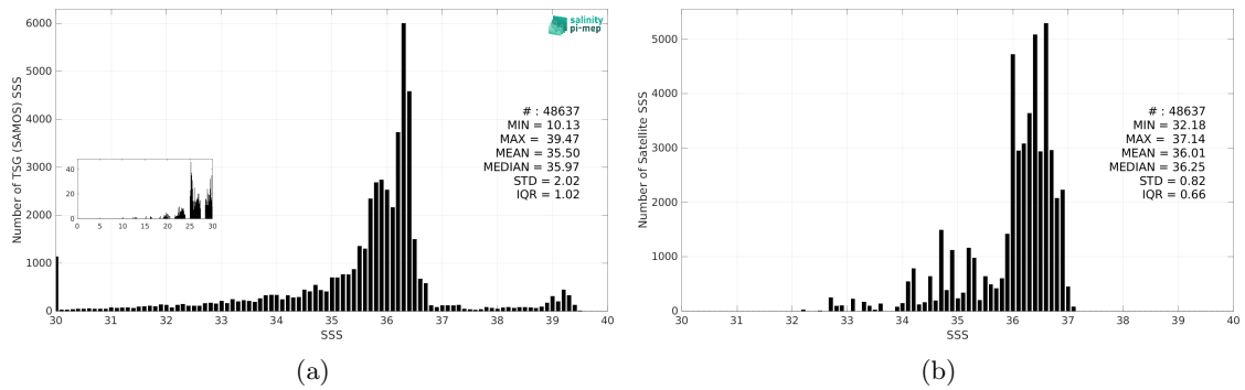
Figure 3: Histograms of SSS from TSG (SAMOS) (a) and Aquarius SSS L3 CAP v5 - Monthly (JPL) (b) considering all match-up pairs per bins of 0.1 over the Mississippi river plume Pi-MEP region and for the full satellite product period.
