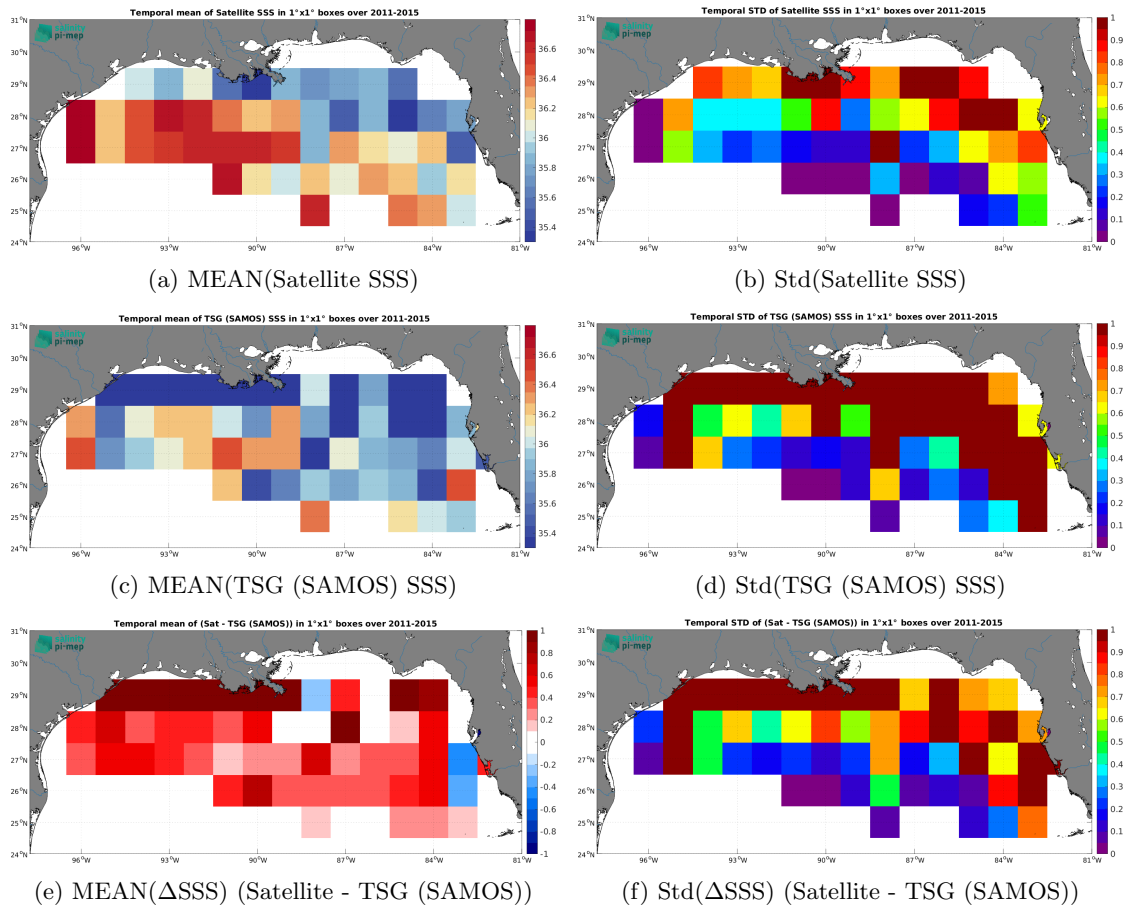
Figure 7: Temporal mean (left) and Std (right) of SSS from Aquarius SSS L3 CAP v5 - Monthly (JPL) (top), TSG (SAMOS) (middle), and of \Delta SSS (Satellite - TSG (SAMOS)). Only match-up pairs are used to generate these maps.
