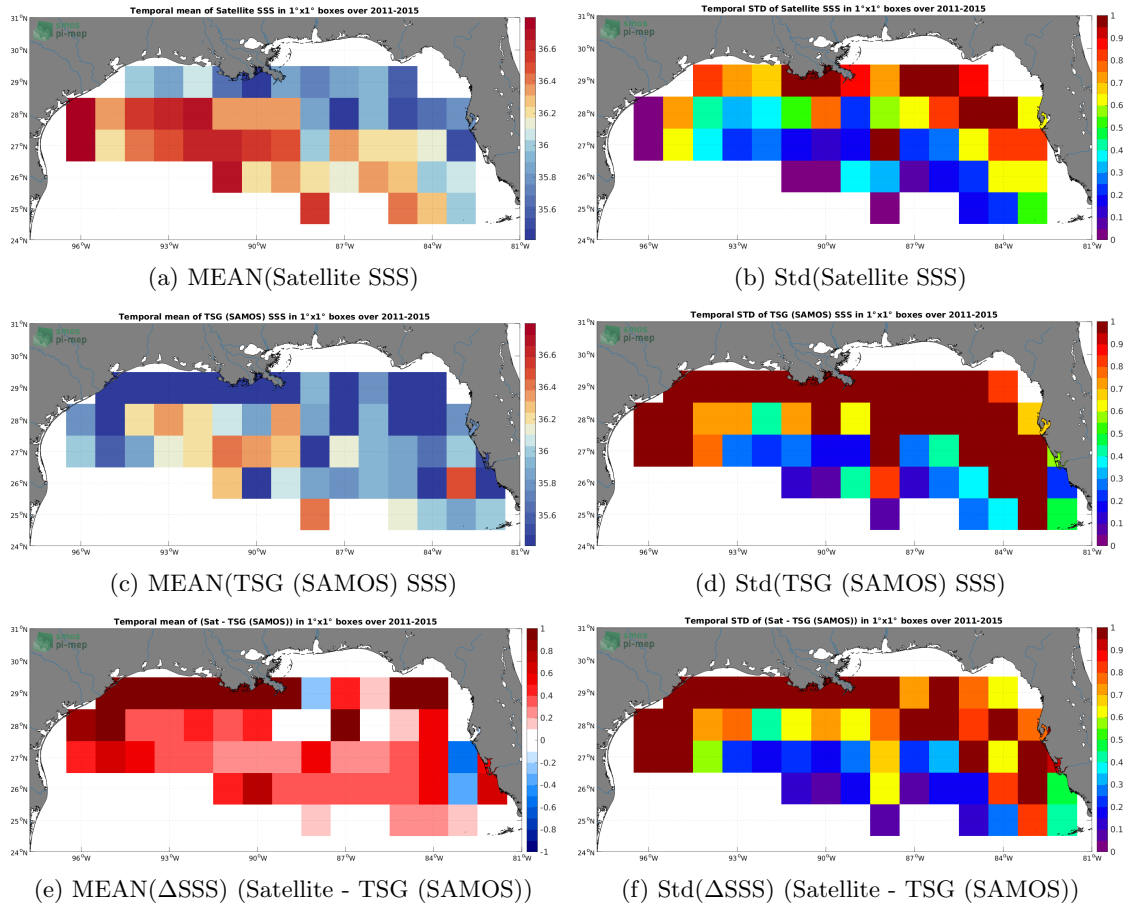
Figure 6: Temporal mean (left) and Std (right) of SSS from Aquarius SSS L3 CAP v5 - Monthly (JPL) (top), TSG (SAMOS) (middle), and of \Delta SSS (Satellite - TSG (SAMOS)). Only match-up pairs are used to generate these maps.
