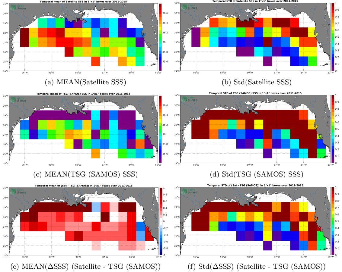
Figure 6: Temporal mean (left) and Std (right) of SSS from Aquarius SSS L3 CAP v5 - Monthly (JPL) (top), TSG (SAMOS) (middle), and of \Delta\text{SSS}(\text{Satellite} - \text{TSG}(\text{SAMOS})) . Only match-up pairs are used to generate these maps.
