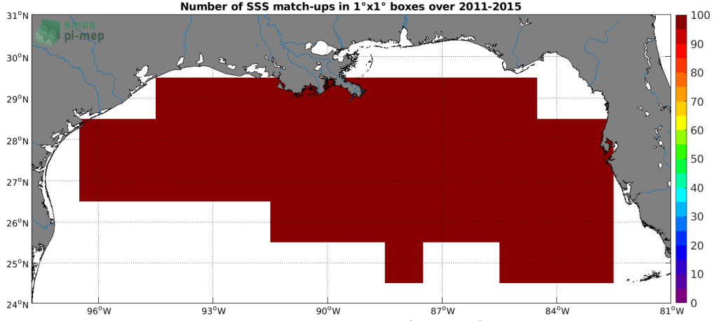
Figure 4: Number of SSS match-ups between TSG (SAMOS) SSS and the Aquarius SSS L3 CAP v5 - Monthly (JPL) SSS product for the Mississippi river plume Pi-MEP region over 1^\circ \times 1^\circ boxes and for the full satellite product period.
