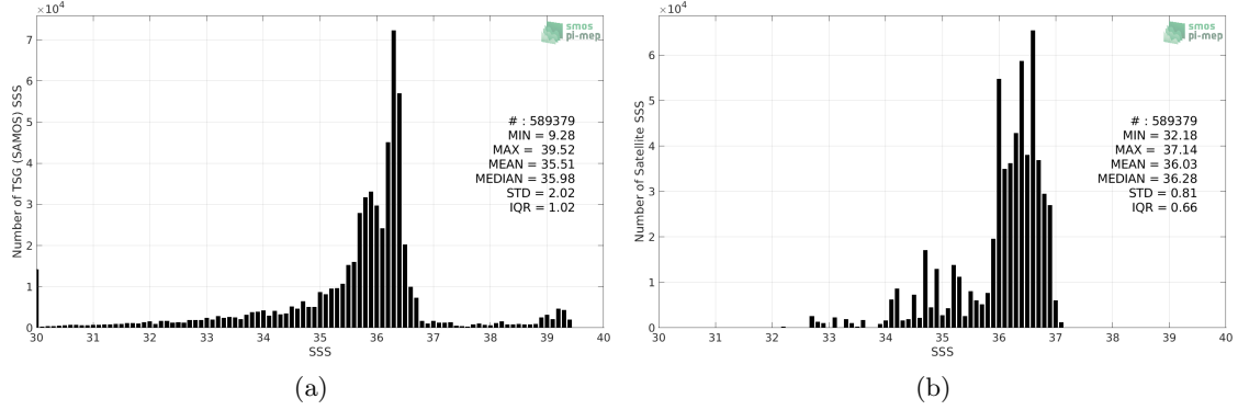
Figure 2: Histograms of SSS from TSG (SAMOS) (a) and Aquarius SSS L3 CAP v5 - Monthly (JPL) (b) considering all match-up pairs per bins of 0.1 over the Mississippi river plume Pi-MEP region and for the full satellite product period.
