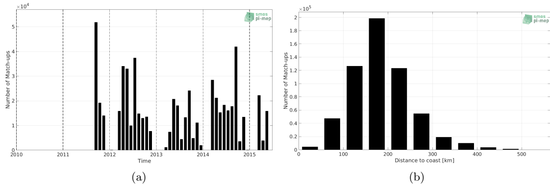
Figure 1: Number of match-ups between TSG (SAMOS) and Aquarius SSS L3 CAP v5 - Monthly (JPL) SSS as a function of time (a) and as function of the distance to coast (b) over the Mississippi river plume Pi-MEP region and for the full satellite product period.
