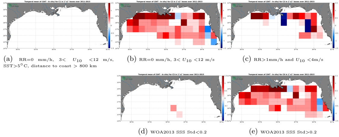
Figure 12: Temporal mean gridded over spatial boxes of size 1^{\circ}\times 1^{\circ} of \Delta\text{SSS} (Aquarius SSS L3 CAP v5 - Monthly (JPL) - TSG (SAMOS)) for 5 different subdatasets corresponding to: \text{RR}=0 mm/h, 3 < U_{10} < 12 m/s, \text{SST} > 5^{\circ}\text{C} , distance to coast > 800 km (a), \text{RR}=0 mm/h, 3 < U_{10} < 12 m/s (b), \text{RR} > 1 mm/h and U_{10} < 4 m/s (c), WOA2013 SSS Std < 0.2 (d), WOA2013 SSS Std > 0.2 (e).
