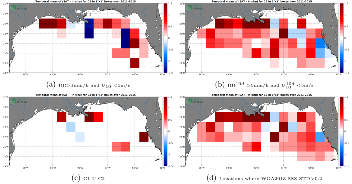
Figure 12: Temporal mean gridded over spatial boxes of size 1^\circ \times 1^\circ of \Delta SSS (Aquarius-L3-JPL-V5-MONTHLY - TSG-SAMOS) for 4 different subdatasets corresponding to: RR > 1\text{mm/h} and U_{10} < 5\text{m/s} (a), RR^{10d} > 5\text{mm/h} and U_{10}^{10d} < 5\text{m/s} (b), C1 U C2 (c), Locations where WOA2013 SSS STD > 0.2 (d).
