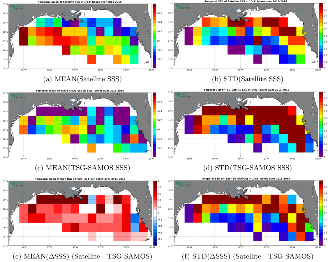
Figure 6: Temporal mean (left) and STD (right) of SSS from Aquarius-L3-JPL-V5-MONTHLY (top), TSG-SAMOS (middle), and of \Delta SSS (Satellite - TSG-SAMOS). Only match-up pairs are used to generate these maps.
