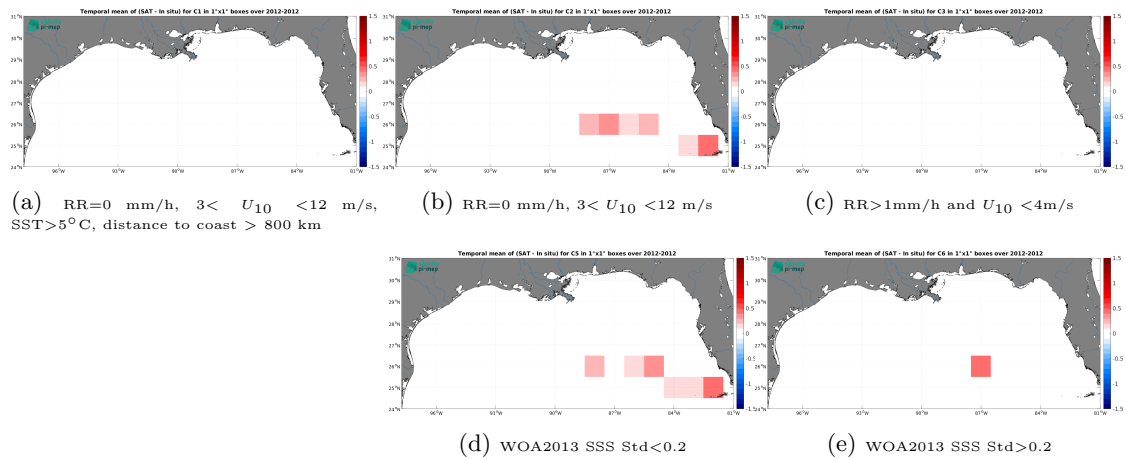
Figure 12: Temporal mean gridded over spatial boxes of size 1^{\circ}\times 1^{\circ} of \Delta SSS (Aquarius SSS L3 CAP v5 - Monthly (JPL) - TSG (GOSUD-Sailing-ship)) for 5 different subdatasets corresponding to:RR=0 mm/h, 3 < U_{10} < 12 m/s, SST >5^{\circ}\text{C} , distance to coast > 800 km (a), RR=0 mm/h, 3 < U_{10} < 12 m/s (b), RR >1 mm/h and U_{10} < 4 m/s (c), WOA2013 SSS Std <0.2 (d), WOA2013 SSS Std >0.2 (e).
