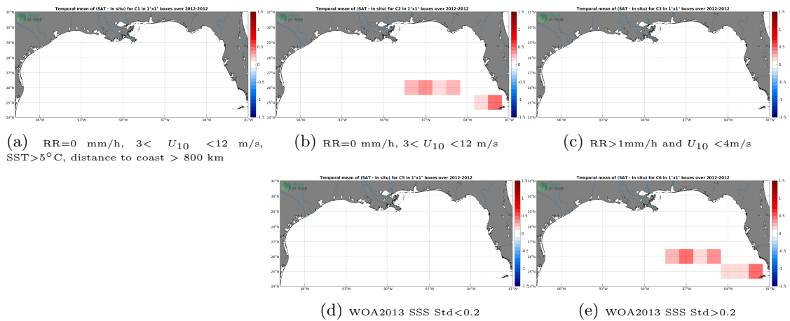
Figure 12: Temporal mean gridded over spatial boxes of size 1^\circ \times 1^\circ of \Delta SSS (Aquarius-L3-JPL-V5-MONTHLY - TSG-GOSUD-Sailing-ship) for 5 different subdatasets corresponding to:RR=0 mm/h, 3 < U_{10} < 12 m/s, SST > 5°C, distance to coast > 800 km (a), RR=0 mm/h, 3 < U_{10} < 12 m/s (b), RR > 1mm/h and U_{10} < 4 m/s (c), WOA2013 SSS Std < 0.2 (d), WOA2013 SSS Std > 0.2 (e).
