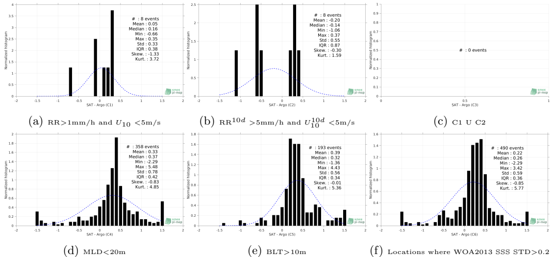
Figure 13: Normalized histogram of \Delta\text{SSS} (Aquarius-L3-JPL-V5-MONTHLY - Argo) for 6 different subdatasets corresponding to: \text{RR} > 1\text{mm/h} and U_{10} < 5\text{m/s} (a), \text{RR}^{10d} > 5\text{mm/h} and U_{10}^{10d} < 5\text{m/s} (b), C1 U C2 (c), \text{MLD} < 20\text{m} (d), \text{BLT} > 10\text{m} (e), Locations where WOA2013 SSS \text{STD} > 0.2 (f).
