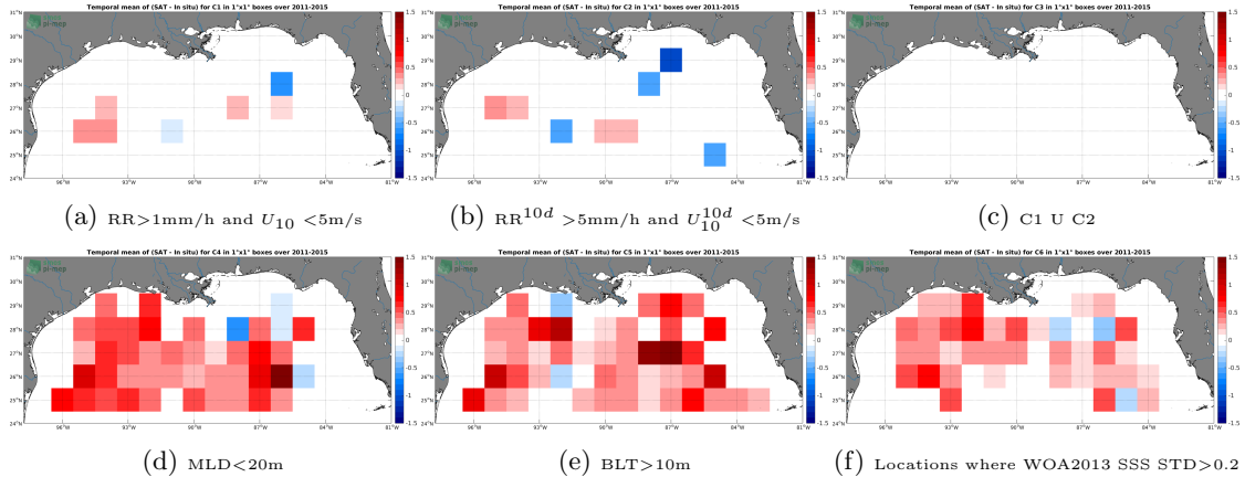
Figure 12: Temporal mean gridded over spatial boxes of size 1^\circ \times 1^\circ of \Delta\text{SSS} (Aquarius-L3-JPL-V5-MONTHLY - Argo) for 6 different subdatasets corresponding to: \text{RR} > 1\text{mm/h} and U_{10} < 5\text{m/s} (a), \text{RR}^{10d} > 5\text{mm/h} and U_{10}^{10d} < 5\text{m/s} (b), C1 U C2 (c), \text{MLD} < 20\text{m} (d), \text{BLT} > 10\text{m} (e), Locations where WOA2013 SSS \text{STD} > 0.2 (f).
