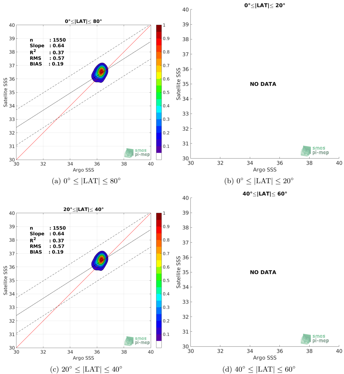
Figure 9: Contour maps of the concentration of Aquarius SSS L2-AVERAGED OR v5 (NASA-GSFC) SSS (y-axis) versus Argo SSS (x-axis) at match-up pairs for different latitude bands. For each plot, the red line shows x=y . The black thin and dashed lines indicate a linear fit through the data cloud and the \pm 95\% confidence levels, respectively. The number match-up pairs n , the slope and R^2 coefficient of the linear fit, the root mean square (RMS) and the mean bias between satellite and in situ data are indicated for each latitude band in each plots.
