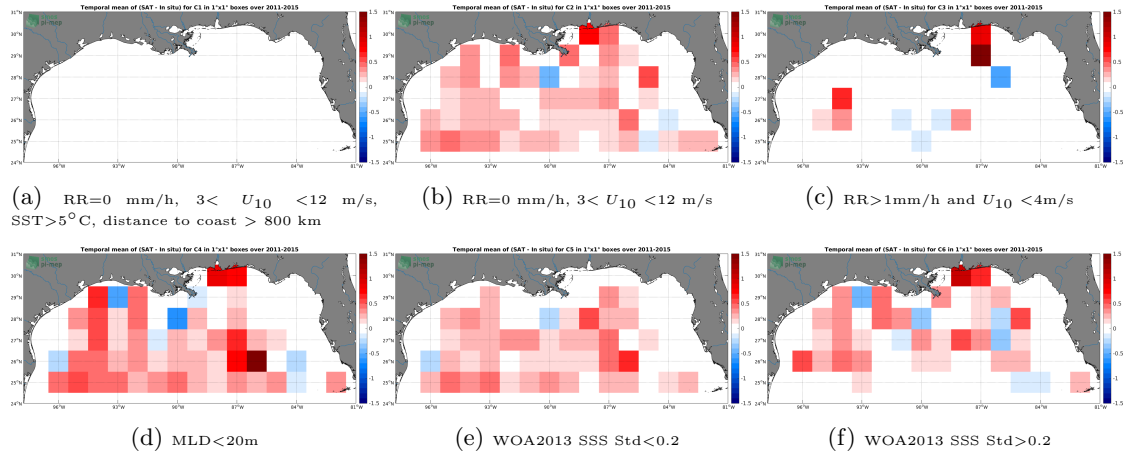
Figure 12: Temporal mean gridded over spatial boxes of size 1^{\circ}\times 1^{\circ} of \Delta\text{SSS} (Aquarius SSS L2-AVERAGED OR v5 (NASA-GSFC) - Argo) for 6 different subdatasets corresponding to: RR=0 mm/h, 3 < U_{10} < 12 m/s, SST > 5^{\circ}\text{C} , distance to coast > 800 km (a), RR=0 mm/h, 3 < U_{10} < 12 m/s (b), RR > 1 mm/h and U_{10} < 4 m/s (c), MLD < 20\text{m} (d), WOA2013 SSS Std < 0.2 (e), WOA2013 SSS Std > 0.2 (f).
