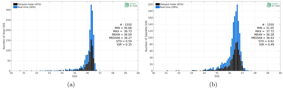
Figure 2: Histograms of SSS from Argos (a) and Aquarius SSS L2-AVERAGED OR v5 (NASA-GSFC) (b) considering all match-up pairs per bins of 0.1 over the Mississippi river plume Pi-MEP region and for the full satellite product period.
