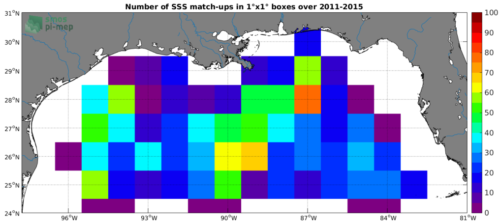
Figure 4: Number of SSS match-ups between Argo SSS and the Aquarius SSS L2-AVERAGED OR v5 (NASA-GSFC) SSS product for the Mississippi river plume Pi-MEP region over 1^\circ \times 1^\circ boxes and for the full satellite product period.
