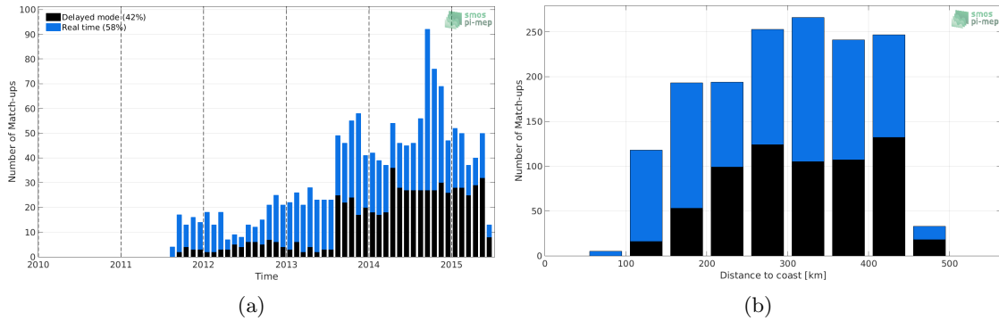
Figure 1: Number of match-ups between Argo and Aquarius SSS L2-AVERAGED OR v5 (NASA-GSFC) SSS as a function of time (a) and as function of the distance to coast (b) over the Mississippi river plume Pi-MEP region and for the full satellite product period.
