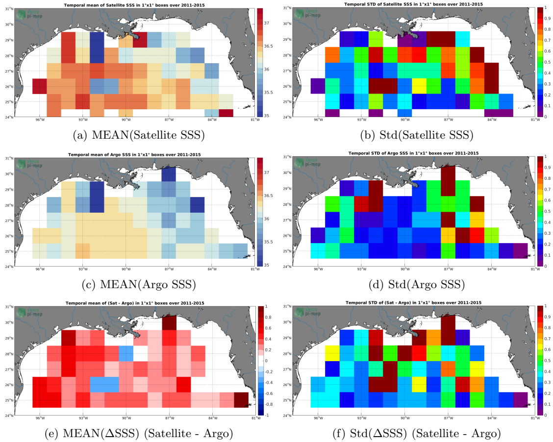
Figure 6: Temporal mean (left) and Std (right) of SSS from Aquarius SSS L2-AVERAGED CAP v5 (JPL) (top), Argo (middle), and of \Delta SSS (Satellite - Argo). Only match-up pairs are used to generate these maps.
