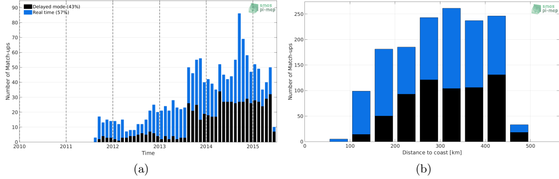
Figure 1: Number of match-ups between Argo and Aquarius SSS L2-AVERAGED CAP v5 (JPL) SSS as a function of time (a) and as function of the distance to coast (b) over the Mississippi river plume Pi-MEP region and for the full satellite product period.
