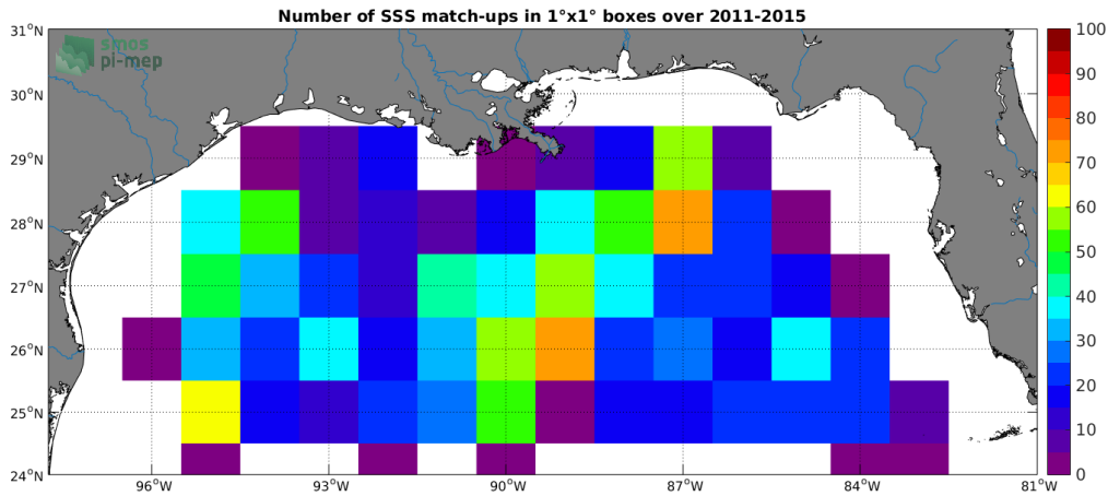
Figure 4: Number of SSS match-ups between Argo SSS and the Aquarius SSS L2-AVERAGED CAP v5 (JPL) SSS product for the Mississippi river plume Pi-MEP region over 1^\circ \times 1^\circ boxes and for the full satellite product period.
