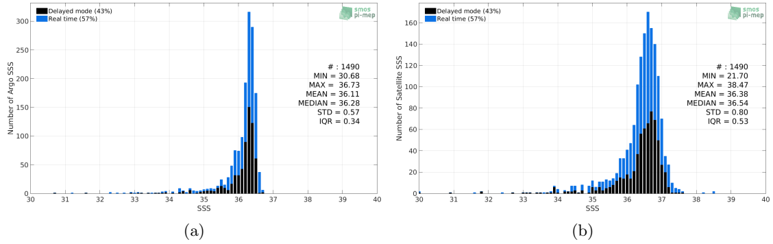
Figure 2: Histograms of SSS from Argo (a) and Aquarius SSS L2-AVERAGED CAP v5 (JPL) (b) considering all match-up pairs per bins of 0.1 over the Mississippi river plume Pi-MEP region and for the full satellite product period.
