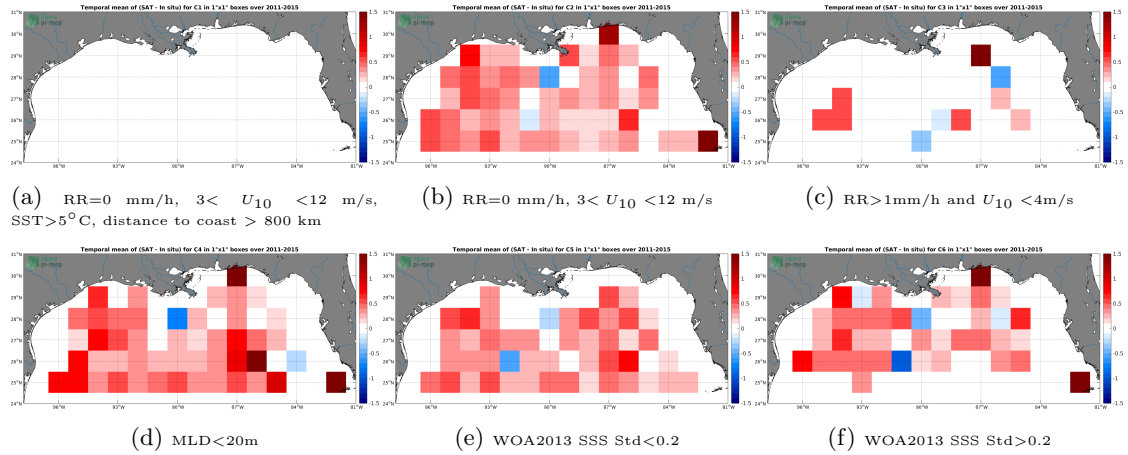
Figure 12: Temporal mean gridded over spatial boxes of size 1^{\circ}\times 1^{\circ} of \Delta\text{SSS} (Aquarius SSS L2-AVERAGED CAP v5 (JPL) - Argo) for 6 different subdatasets corresponding to:RR=0 mm/h, 3 < U_{10} < 12 m/s, SST >5^{\circ}\text{C} , distance to coast > 800 km (a), RR=0 mm/h, 3 < U_{10} < 12 m/s (b), RR >1 mm/h and U_{10} < 4 m/s (c),MLD <20 m (d),WOA2013 SSS Std <0.2 (e),WOA2013 SSS Std >0.2 (f).
