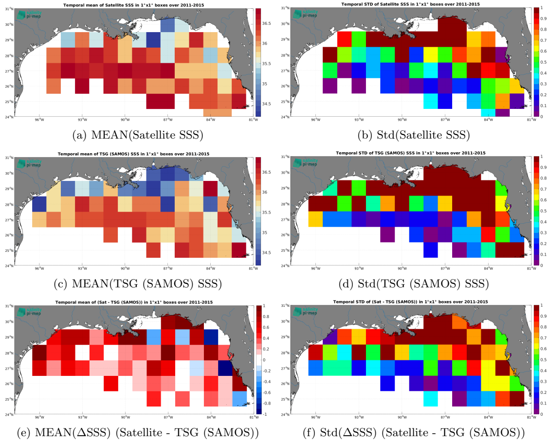
Figure 7: Temporal mean (left) and Std (right) of SSS from Aquarius SSS L2 OR v5 (NASA-GSFC) (top), TSG (SAMOS) (middle), and of \Delta SSS (Satellite - TSG (SAMOS)). Only match-up pairs are used to generate these maps.
