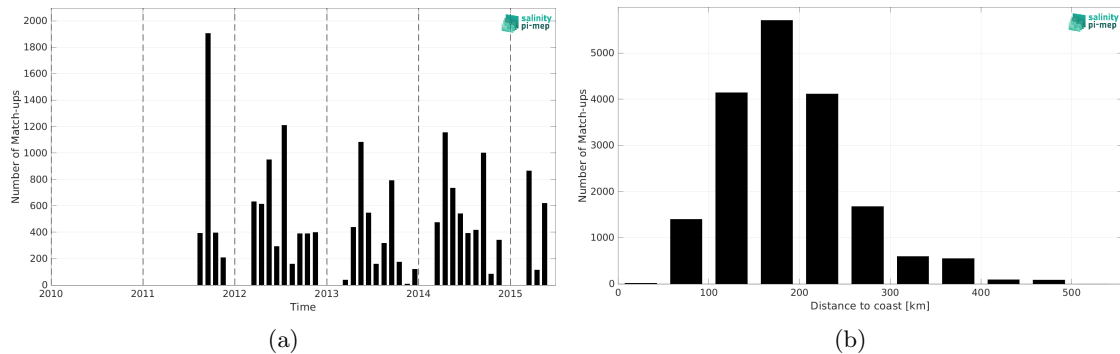
Figure 2: Number of match-ups between TSG (SAMOS) and Aquarius SSS L2 OR v5 (NASA-GSFC) SSS as a function of time (a) and as function of the distance to coast (b) over the Mississippi river plume Pi-MEP region and for the full satellite product period.
