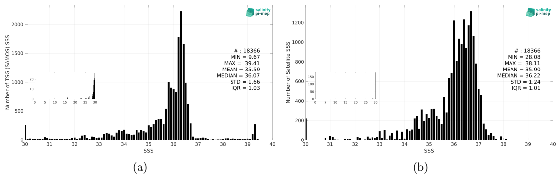
Figure 3: Histograms of SSS from TSG (SAMOS) (a) and Aquarius SSS L2 OR v5 (NASA-GSFC) (b) considering all match-up pairs per bins of 0.1 over the Mississippi river plume Pi-MEP region and for the full satellite product period.
