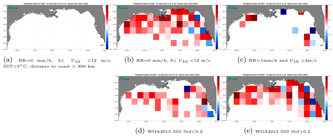
Figure 14: Temporal mean gridded over spatial boxes of size 1^\circ \times 1^\circ of \Delta SSS (Aquarius SSS L2 OR v5 (NASA-GSFC) - TSG (SAMOS)) for 5 different subdatasets corresponding to:RR=0 mm/h, 3 < U_{10} < 12 m/s, SST > 5^\circ C , distance to coast > 800 km (a), RR=0 mm/h, 3 < U_{10} < 12 m/s (b), RR>1mm/h and U_{10} < 4 m/s (c), WOA2013 SSS Std<0.2 (d), WOA2013 SSS Std>0.2 (e).
