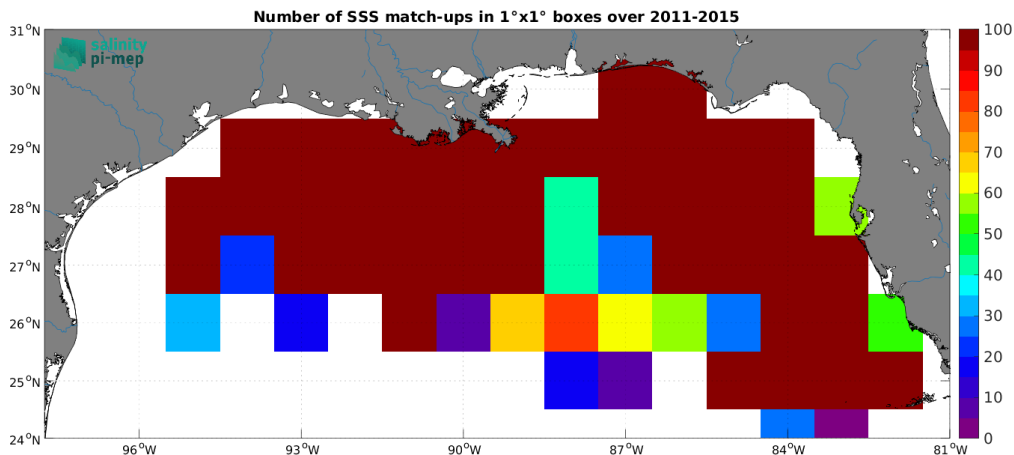
Figure 5: Number of SSS match-ups between TSG (SAMOS) SSS and the Aquarius SSS L2 OR v5 (NASA-GSFC) SSS product for the Mississippi river plume Pi-MEP region over 1^\circ \times 1^\circ boxes and for the full satellite product period.
