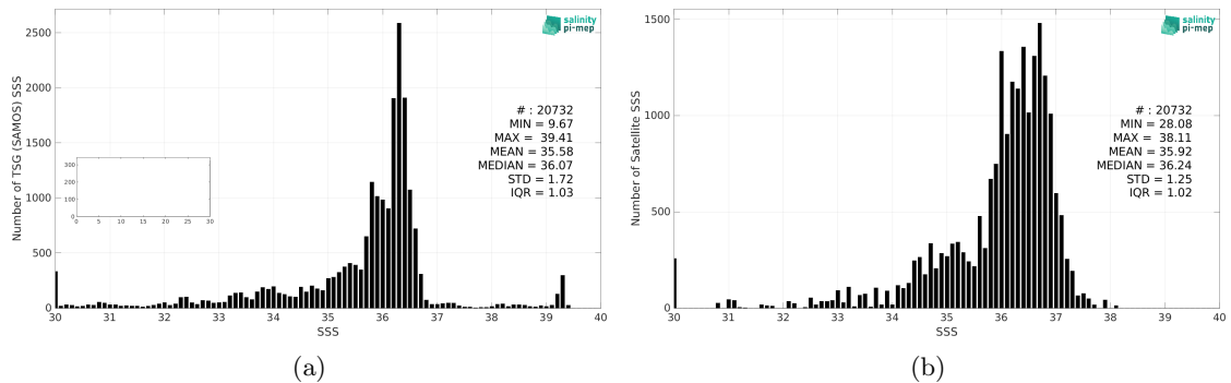
Figure 2: Histograms of SSS from TSG (SAMOS) (a) and Aquarius SSS L2 OR v5 (NASA-GSFC) (b) considering all match-up pairs per bins of 0.1 over the Mississippi river plume Pi-MEP region and for the full satellite product period.
