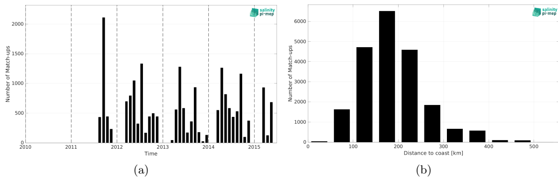
Figure 1: Number of match-ups between TSG (SAMOS) and Aquarius SSS L2 OR v5 (NASA-GSFC) SSS as a function of time (a) and as function of the distance to coast (b) over the Mississippi river plume Pi-MEP region and for the full satellite product period.
