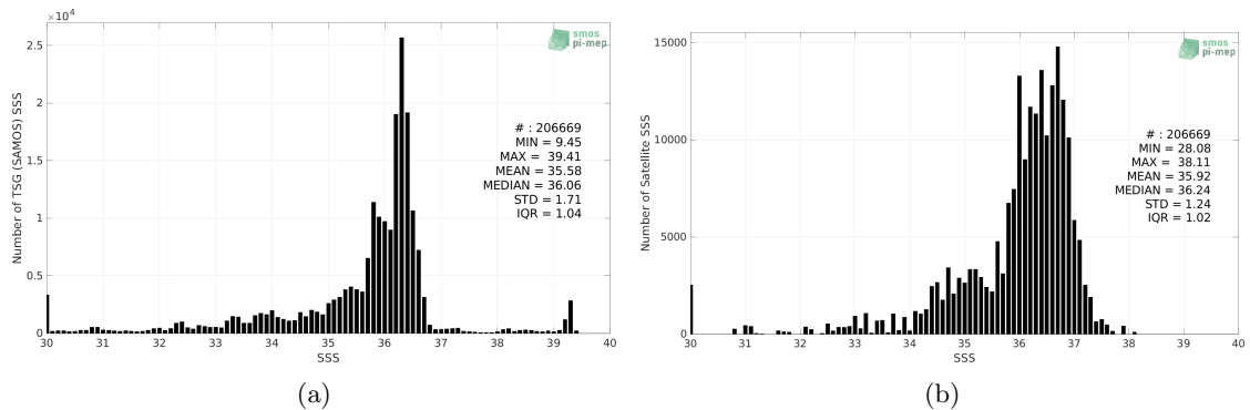
Figure 2: Histograms of SSS from TSG (SAMOS) (a) and Aquarius SSS L2 OR v5 (NASA-GSFC) (b) considering all match-up pairs per bins of 0.1 over the Mississippi river plume Pi-MEP region and for the full satellite product period.
