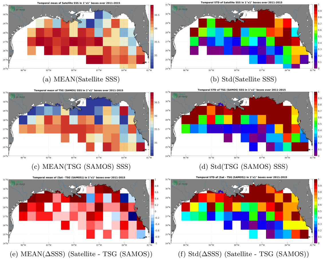
Figure 6: Temporal mean (left) and Std (right) of SSS from Aquarius SSS L2 OR v5 (NASA-GSFC) (top), TSG (SAMOS) (middle), and of \Delta SSS (Satellite - TSG (SAMOS)). Only match-up pairs are used to generate these maps.
