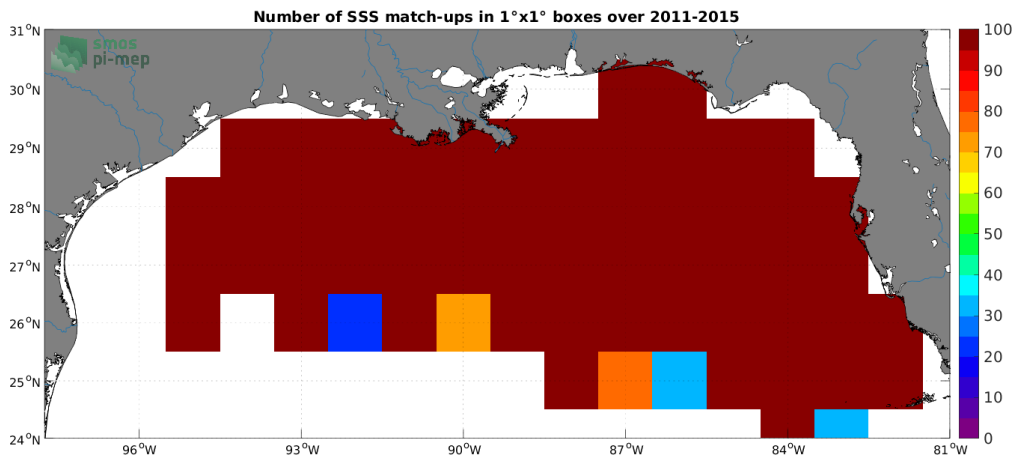
Figure 4: Number of SSS match-ups between TSG (SAMOS) SSS and the Aquarius SSS L2 OR v5 (NASA-GSFC) SSS product for the Mississippi river plume Pi-MEP region over 1^\circ \times 1^\circ boxes and for the full satellite product period.
