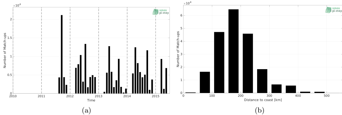
Figure 1: Number of match-ups between TSG (SAMOS) and Aquarius SSS L2 OR v5 (NASA-GSFC) SSS as a function of time (a) and as function of the distance to coast (b) over the Mississippi river plume Pi-MEP region and for the full satellite product period.
