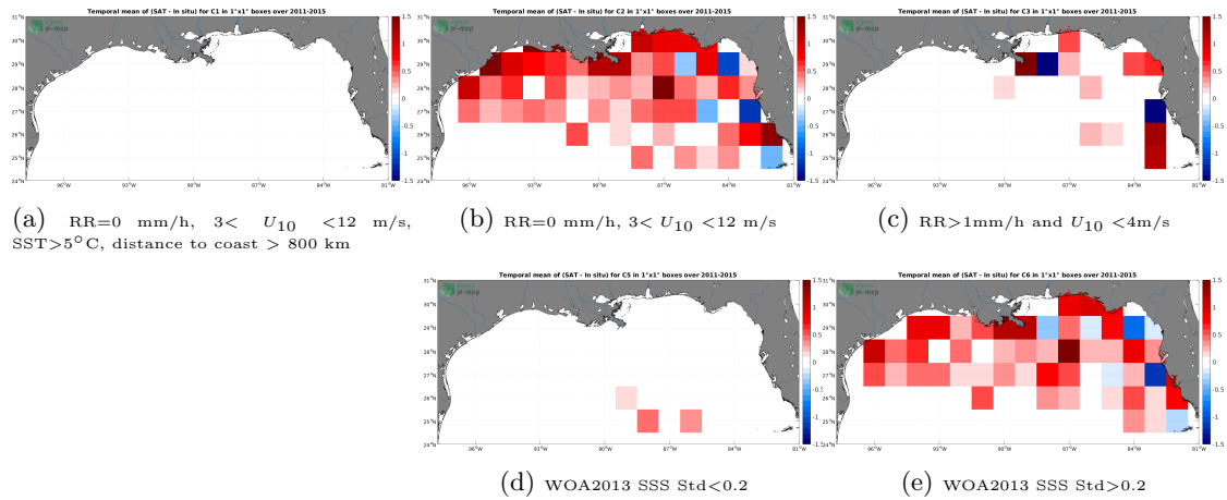
Figure 12: Temporal mean gridded over spatial boxes of size 1^{\circ}\times 1^{\circ} of \Delta\text{SSS} (Aquarius SSS L2 OR v5 (NASA-GSFC) - TSG (SAMOS)) for 5 different subdatasets corresponding to:RR=0 mm/h, 3 < U_{10} < 12 m/s, SST >5^{\circ}\text{C} , distance to coast > 800 km (a), RR=0 mm/h, 3 < U_{10} < 12 m/s (b), RR >1 mm/h and U_{10} < 4 m/s (c), WOA2013 SSS Std <0.2 (d), WOA2013 SSS Std >0.2 (e).
