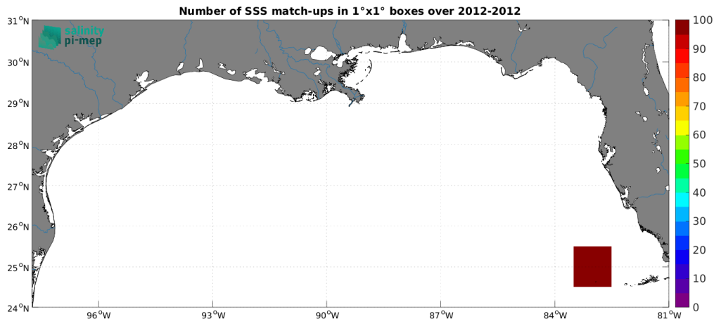
Figure 5: Number of SSS match-ups between TSG (GOSUD-Sailing-ship) SSS and the Aquarius SSS L2 OR v5 (NASA-GSFC) SSS product for the Mississippi river plume Pi-MEP region over 1^\circ \times 1^\circ boxes and for the full satellite product period.
