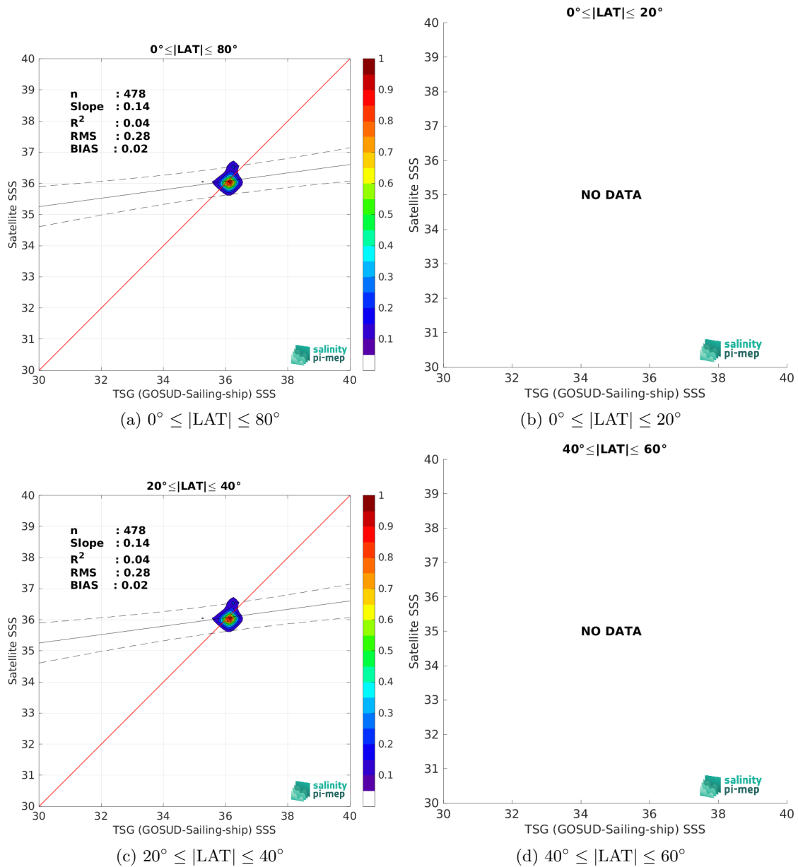
Figure 10: Contour maps of the concentration of Aquarius SSS L2 OR v5 (NASA-GSFC) SSS (y-axis) versus TSG (GOSUD-Sailing-ship) SSS (x-axis) at match-up pairs for different latitude bands. For each plot, the red line shows x=y . The black thin and dashed lines indicate a linear fit through the data cloud and the \pm 95\% confidence levels, respectively. The number match-up pairs n , the slope and R^2 coefficient of the linear fit, the root mean square (RMS) and the mean bias between satellite and in situ data are indicated for each latitude band in each plots.
