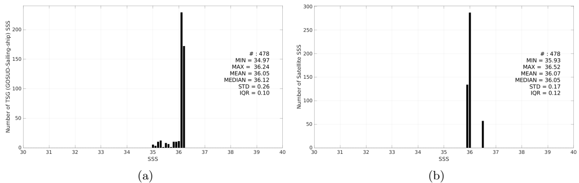
Figure 3: Histograms of SSS from TSG (GOSUD-Sailing-ship) (a) and Aquarius SSS L2 OR v5 (NASA-GSFC) (b) considering all match-up pairs per bins of 0.1 over the Mississippi river plume Pi-MEP region and for the full satellite product period.
