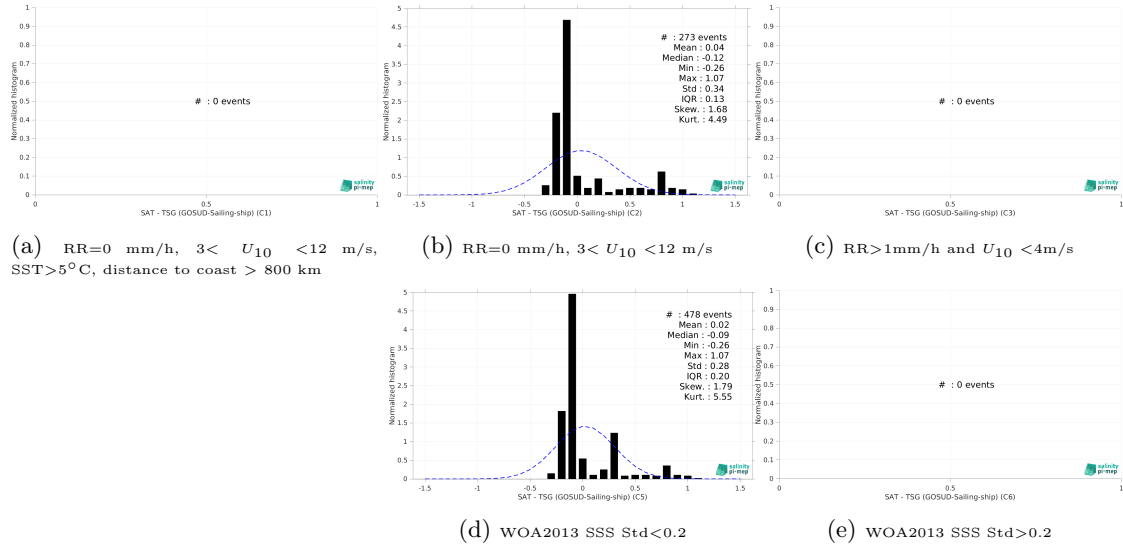
Figure 15: Normalized histogram of \Delta SSS (Aquarius SSS L2 OR v5 (NASA-GSFC) - TSG (GOSUD-Sailing-ship)) for 5 different subdatasets corresponding to: RR=0 mm/h, 3 < U_{10} < 12 m/s, SST > 5°C, distance to coast > 800 km (a), RR=0 mm/h, 3 < U_{10} < 12 m/s (b), RR > 1mm/h and U_{10} < 4 m/s (c), WOA2013 SSS Std < 0.2 (d), WOA2013 SSS Std > 0.2 (e).
