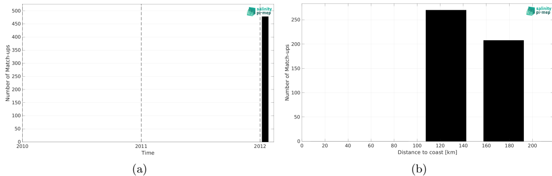
Figure 2: Number of match-ups between TSG (GOSUD-Sailing-ship) and Aquarius SSS L2 OR v5 (NASA-GSFC) SSS as a function of time (a) and as function of the distance to coast (b) over the Mississippi river plume Pi-MEP region and for the full satellite product period.
