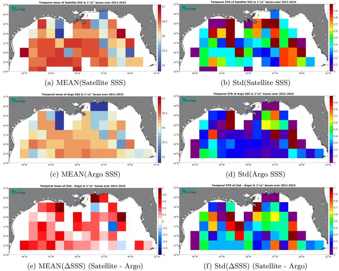
Figure 7: Temporal mean (left) and Std (right) of SSS from Aquarius SSS L2 OR v5 (NASA-GSFC) (top), Argo (middle), and of \Delta\text{SSS} (Satellite - Argo). Only match-up pairs are used to generate these maps.
