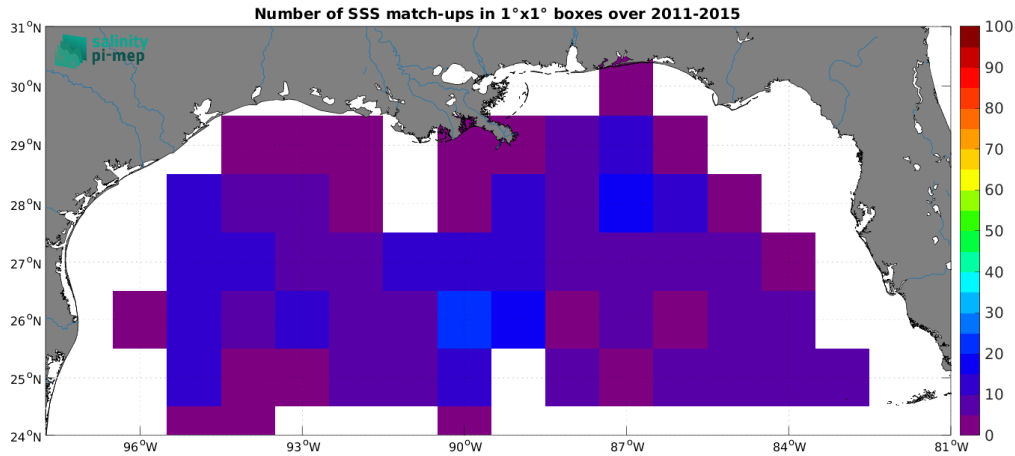
Figure 5: Number of SSS match-ups between Argo SSS and the Aquarius SSS L2 OR v5 (NASA-GSFC) SSS product for the Mississippi river plume Pi-MEP region over 1^\circ \times 1^\circ boxes and for the full satellite product period.
