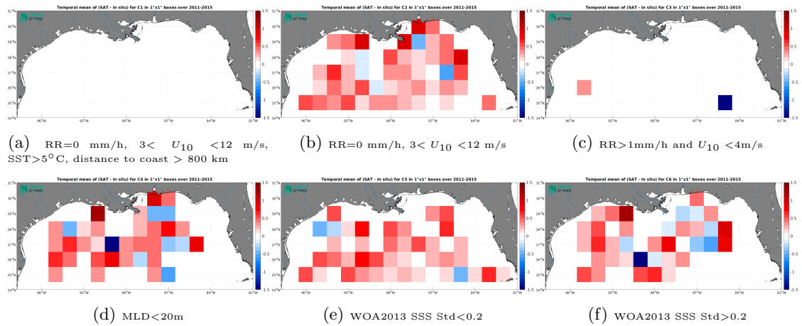
Figure 14: Temporal mean gridded over spatial boxes of size 1^\circ \times 1^\circ of \Delta SSS (Aquarius SSS L2 OR v5 (NASA-GSFC) - Argo) for 6 different subdatasets corresponding to: RR=0 mm/h, 3 < U_{10} < 12 m/s, SST > 5°C, distance to coast > 800 km (a), RR=0 mm/h, 3 < U_{10} < 12 m/s (b), RR > 1mm/h and U_{10} < 4 m/s (c), MLD < 20m (d), WOA2013 SSS Std < 0.2 (e), WOA2013 SSS Std > 0.2 (f).
