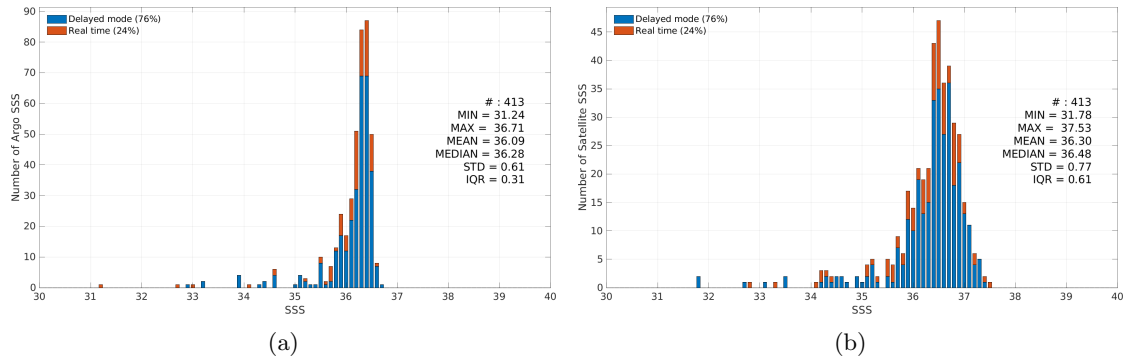
Figure 3: Histograms of SSS from Argo (a) and Aquarius SSS L2 OR v5 (NASA-GSFC) (b) considering all match-up pairs per bins of 0.1 over the Mississippi river plume Pi-MEP region and for the full satellite product period.
