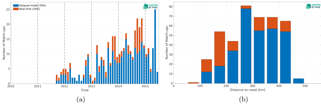
Figure 2: Number of match-ups between Argo and Aquarius SSS L2 OR v5 (NASA-GSFC) SSS as a function of time (a) and as function of the distance to coast (b) over the Mississippi river plume Pi-MEP region and for the full satellite product period.
