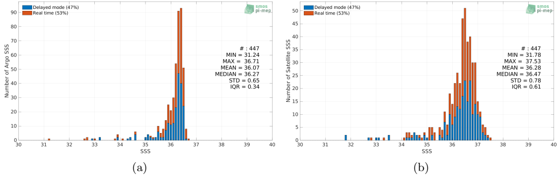
Figure 2: Histograms of SSS from Argo (a) and Aquarius SSS L2 OR v5 (NASA-GSFC) (b) considering all match-up pairs per bins of 0.1 over the Mississippi river plume Pi-MEP region and for the full satellite product period.
