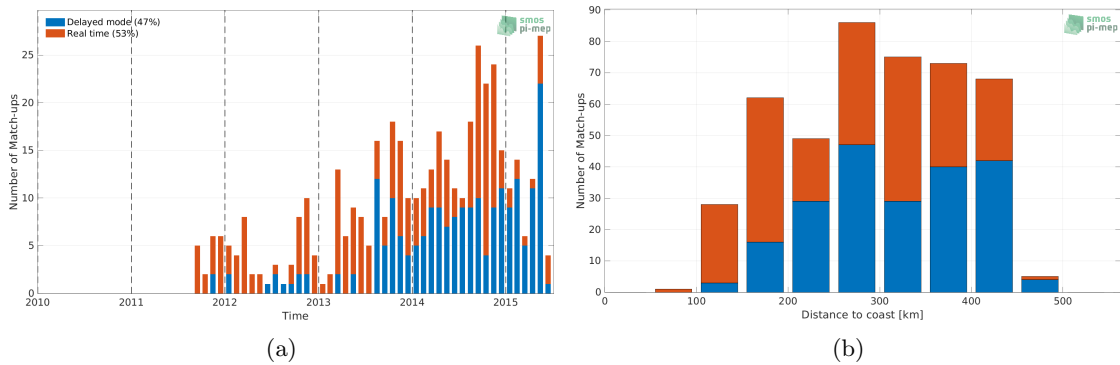
Figure 1: Number of match-ups between Argo and Aquarius SSS L2 OR v5 (NASA-GSFC) SSS as a function of time (a) and as function of the distance to coast (b) over the Mississippi river plume Pi-MEP region and for the full satellite product period.
