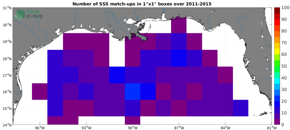
Figure 4: Number of SSS match-ups between Argo SSS and the Aquarius SSS L2 OR v5 (NASA-GSFC) SSS product for the Mississippi river plume Pi-MEP region over 1^\circ \times 1^\circ boxes and for the full satellite product period.
