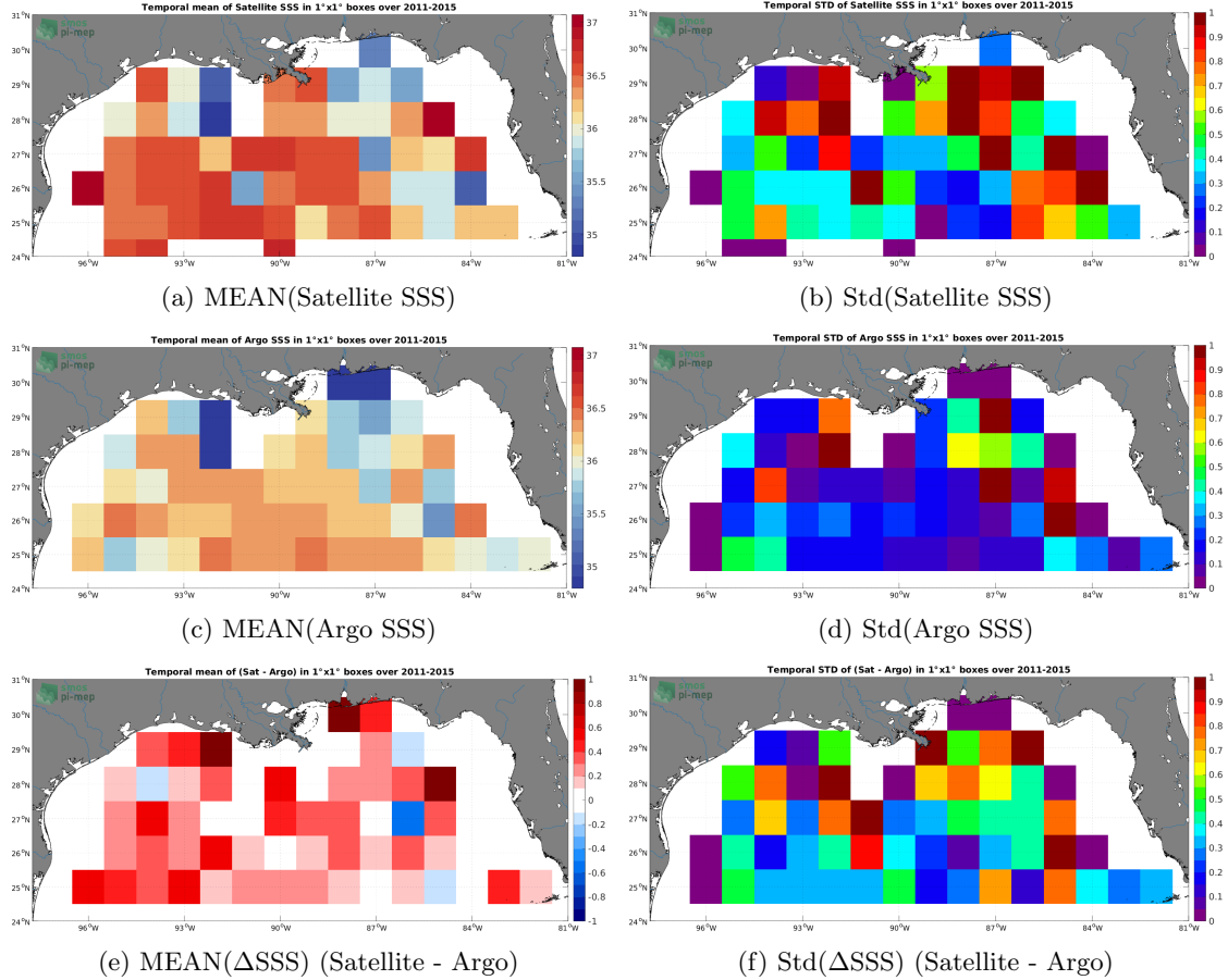
Figure 6: Temporal mean (left) and Std (right) of SSS from Aquarius SSS L2 OR v5 (NASA-GSFC) (top), Argo (middle), and of \Delta\text{SSS} (Satellite - Argo). Only match-up pairs are used to generate these maps.
