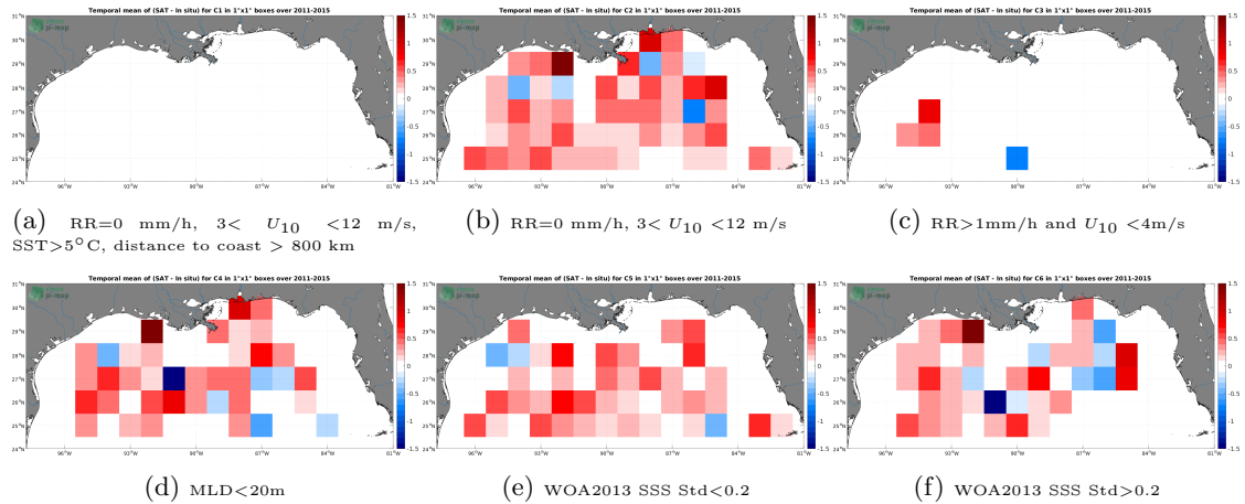
Figure 12: Temporal mean gridded over spatial boxes of size 1^{\circ}\times 1^{\circ} of \Delta\text{SSS} (Aquarius SSS L2 OR v5 (NASA-GSFC) - Argo) for 6 different subdatasets corresponding to:RR=0 mm/h, 3 < U_{10} < 12 m/s, SST > 5^{\circ}\text{C} , distance to coast > 800 km (a), RR=0 mm/h, 3 < U_{10} < 12 m/s (b), RR > 1\text{mm/h} and U_{10} < 4\text{m/s} (c),MLD < 20\text{m} (d),WOA2013 SSS Std < 0.2 (e),WOA2013 SSS Std > 0.2 (f).
