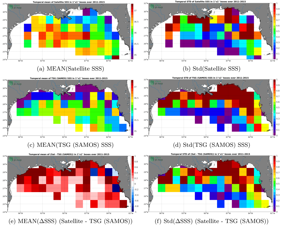
Figure 6: Temporal mean (left) and Std (right) of SSS from Aquarius SSS L2 CAP v5 (JPL) (top), TSG (SAMOS) (middle), and of \Delta SSS (Satellite - TSG (SAMOS)). Only match-up pairs are used to generate these maps.
