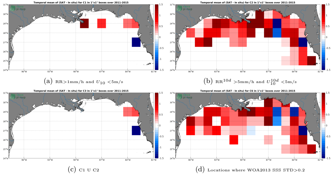
Figure 12: Temporal mean gridded over spatial boxes of size 1^\circ \times 1^\circ of \Delta SSS (Aquarius-L2-JPL-V5 - TSG-SAMOS) for 4 different subdatasets corresponding to: RR > 1\text{mm/h} and U_{10} < 5\text{m/s} (a), RR^{10d} > 5\text{mm/h} and U_{10}^{10d} < 5\text{m/s} (b), C1 U C2 (c), Locations where WOA2013 SSS STD > 0.2 (d).
