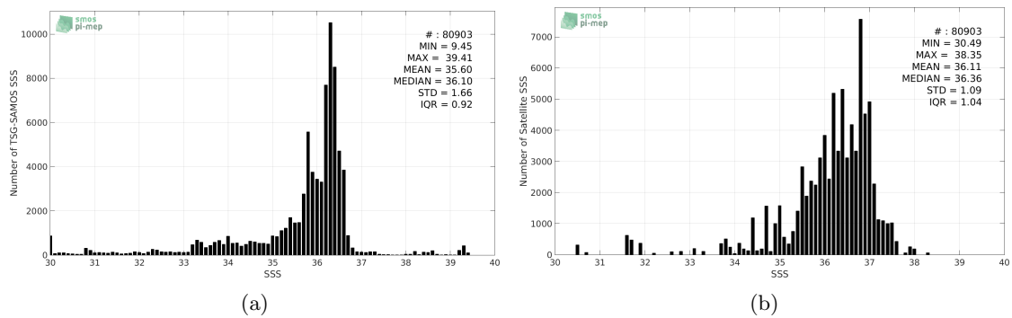
Figure 2: Histograms of SSS from TSG-SAMOS (a) and Aquarius-L2-JPL-V5 (b) considering all match-up pairs per bins of 0.1 over the Mississippi river plume Pi-MEP region and for the full satellite product period.
