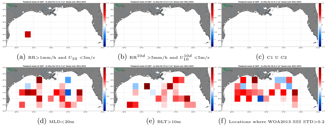
Figure 12: Temporal mean gridded over spatial boxes of size 1^\circ \times 1^\circ of \Delta SSS (Aquarius-L2-JPL-V5 - Argo) for 6 different subdatasets corresponding to: RR > 1\text{mm/h} and U_{10} < 5\text{m/s} (a), RR^{10d} > 5\text{mm/h} and U_{10}^{10d} < 5\text{m/s} (b), C1 U C2 (c), MLD < 20\text{m} (d), BLT > 10\text{m} (e), Locations where WOA2013 SSS STD > 0.2 (f).
