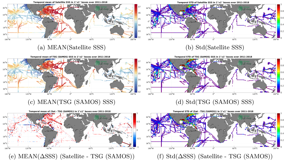
Figure 6: Temporal mean (left) and Std (right) of SSS from SMOS and SMAP SSS L4 OI v1 - 7 Days (LOPS) (top), TSG (SAMOS) (middle), and of \Delta SSS (Satellite - TSG (SAMOS)). Only match-up pairs are used to generate these maps.
