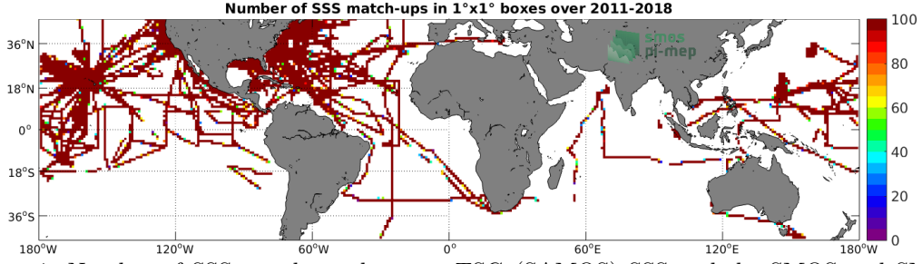
Figure 4: Number of SSS match-ups between TSG (SAMOS) SSS and the SMOS and SMAP SSS L4 OI v1 - 7 Days (LOPS) SSS product for the Mid-Low Latitudes 45N-45S Pi-MEP region over 1^\circ \times 1^\circ boxes and for the full satellite product period.
