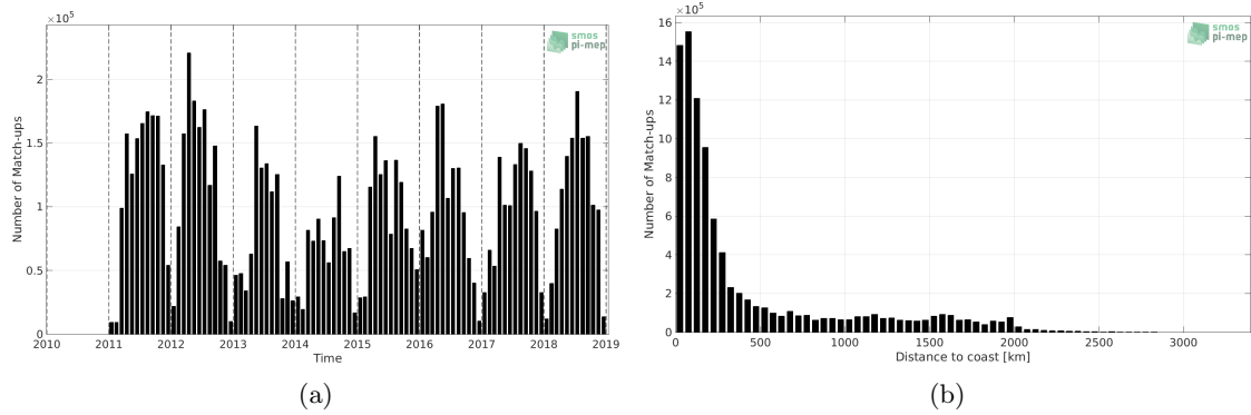
Figure 1: Number of match-ups between TSG (SAMOS) and SMOS and SMAP SSS L4 OI v1 - 7 Days (LOPS) SSS as a function of time (a) and as function of the distance to coast (b) over the Mid-Low Latitudes 45N-45S Pi-MEP region and for the full satellite product period.
