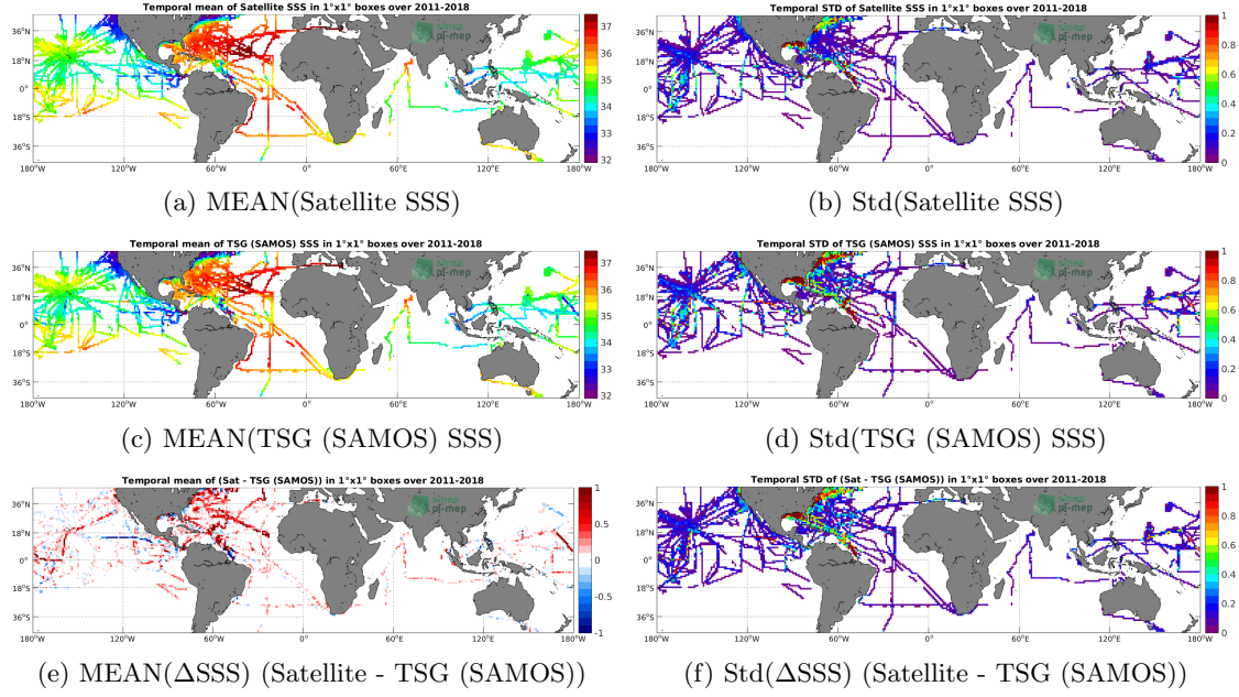
Figure 6: Temporal mean (left) and Std (right) of SSS from SMOS and SMAP SSS L4 OI v1 - 7 Days (LOPS) (top), TSG (SAMOS) (middle), and of \Delta SSS (Satellite - TSG (SAMOS)). Only match-up pairs are used to generate these maps.
