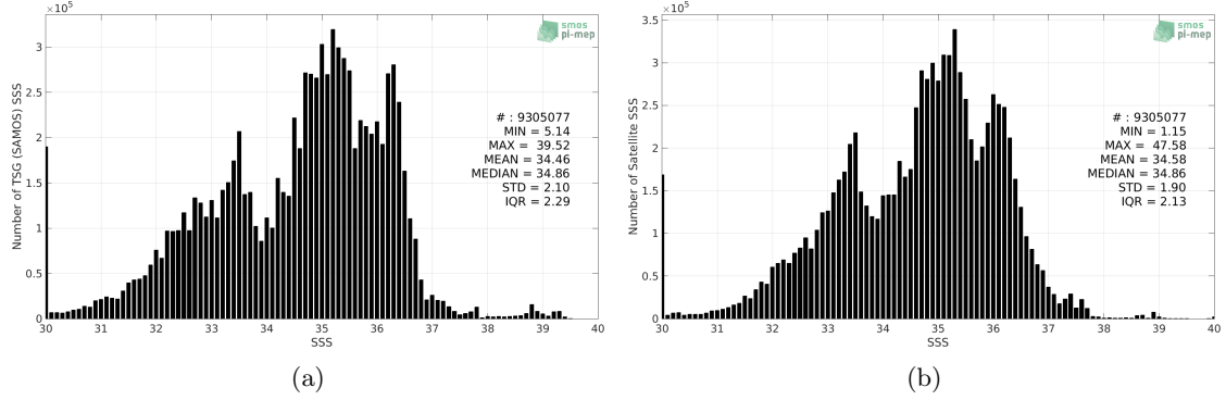
Figure 2: Histograms of SSS from TSG (SAMOS) (a) and SMOS and SMAP SSS L4 OI v1 - 7 Days (LOPS) (b) considering all match-up pairs per bins of 0.1 over the Mid-Low Latitudes 45N-45S Pi-MEP region and for the full satellite product period.
