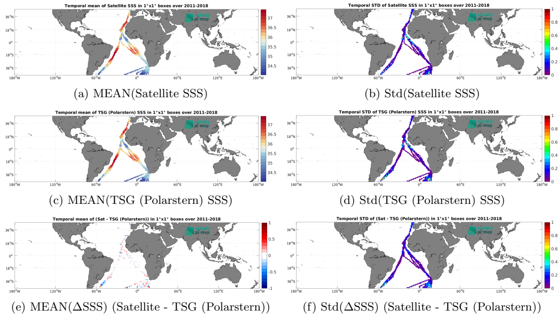
Figure 6: Temporal mean (left) and Std (right) of SSS from SMOS and SMAP SSS L4 OI v1 - 7 Days (LOPS) (top), TSG (Polarstern) (middle), and of \Delta SSS (Satellite - TSG (Polarstern)). Only match-up pairs are used to generate these maps.
