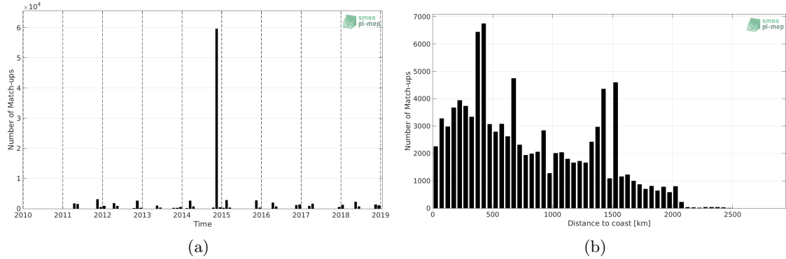
Figure 1: Number of match-ups between TSG (Polarstern) and SMOS and SMAP SSS L4 OI v1 - 7 Days (LOPS) SSS as a function of time (a) and as function of the distance to coast (b) over the Mid-Low Latitudes 45N-45S Pi-MEP region and for the full satellite product period.
