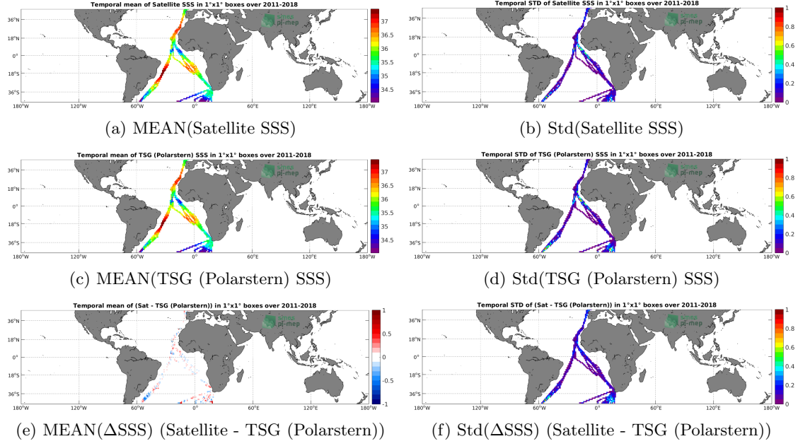
Figure 6: Temporal mean (left) and Std (right) of SSS from SMOS and SMAP SSS L4 OI v1 - 7 Days (LOPS) (top), TSG (Polarstern) (middle), and of \Delta SSS (Satellite - TSG (Polarstern)). Only match-up pairs are used to generate these maps.
