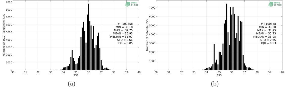
Figure 2: Histograms of SSS from TSG (Polarstern) (a) and SMOS and SMAP SSS L4 OI v1 - 7 Days (LOPS) (b) considering all match-up pairs per bins of 0.1 over the Mid-Low Latitudes 45N-45S Pi-MEP region and for the full satellite product period.
