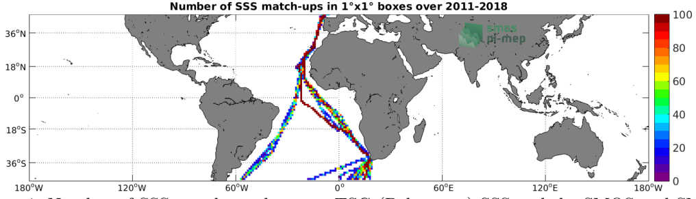
Figure 4: Number of SSS match-ups between TSG (Polarstern) SSS and the SMOS and SMAP SSS L4 OI v1 - 7 Days (LOPS) SSS product for the Mid-Low Latitudes 45N-45S Pi-MEP region over 1^\circ \times 1^\circ boxes and for the full satellite product period.
