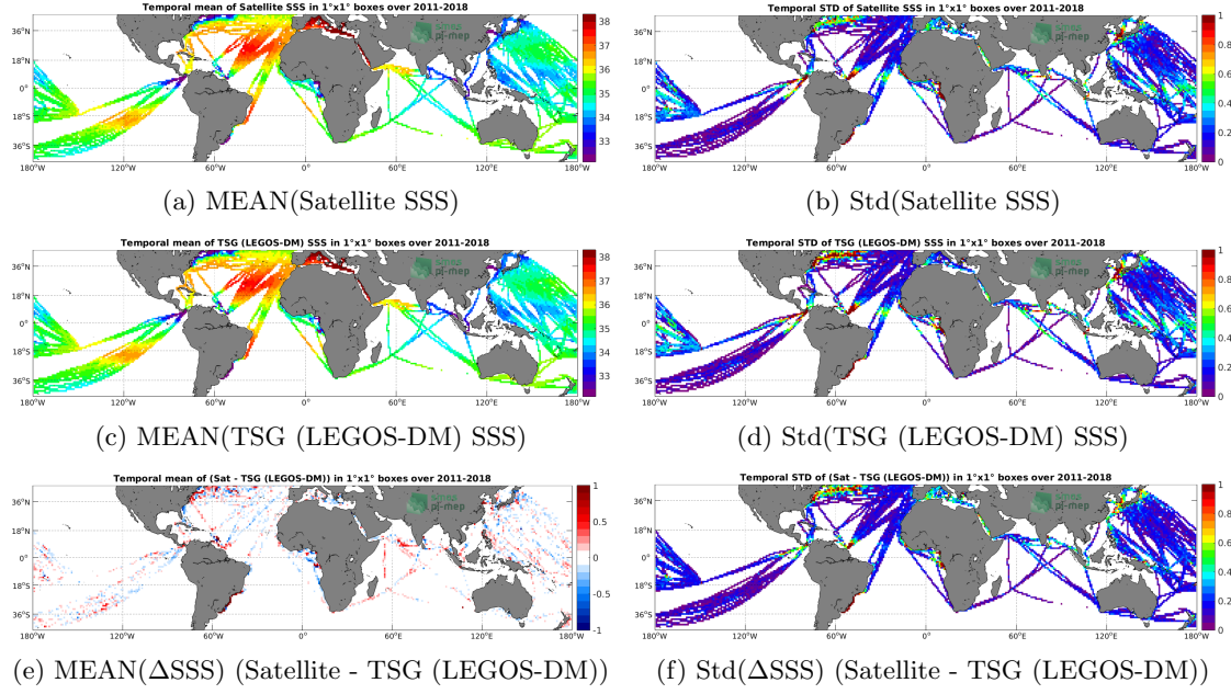
Figure 6: Temporal mean (left) and Std (right) of SSS from SMOS and SMAP SSS L4 OI v1 - 7 Days (LOPS) (top), TSG (LEGOS-DM) (middle), and of \Delta SSS (Satellite - TSG (LEGOS-DM)). Only match-up pairs are used to generate these maps.
