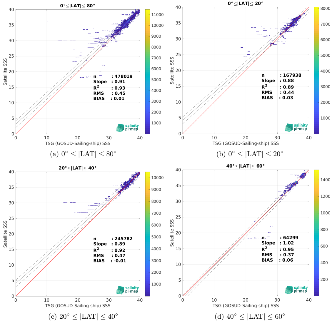
Figure 9: Contour maps of the concentration of SMOS and SMAP SSS L4 OI v1 - 7 Days (LOPS) SSS (y-axis) versus TSG (GOSUD-Sailing-ship) SSS (x-axis) at match-up pairs for different latitude bands. For each plot, the red line shows x=y . The black thin and dashed lines indicate a linear fit through the data cloud and the \pm 95\% confidence levels, respectively. The number of match-up pairs n , the slope and R^2 coefficient of the linear fit, the root mean square (RMS) and the mean bias between satellite and in situ data are indicated for each latitude band in each plot.
