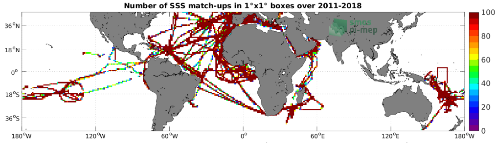
Figure 4: Number of SSS match-ups between TSG (GOSUD-Research-vessel) SSS and the SMOS and SMAP SSS L4 OI v1 - 7 Days (LOPS) SSS product for the Mid-Low Latitudes 45N-45S Pi-MEP region over 1^\circ \times 1^\circ boxes and for the full satellite product period.
