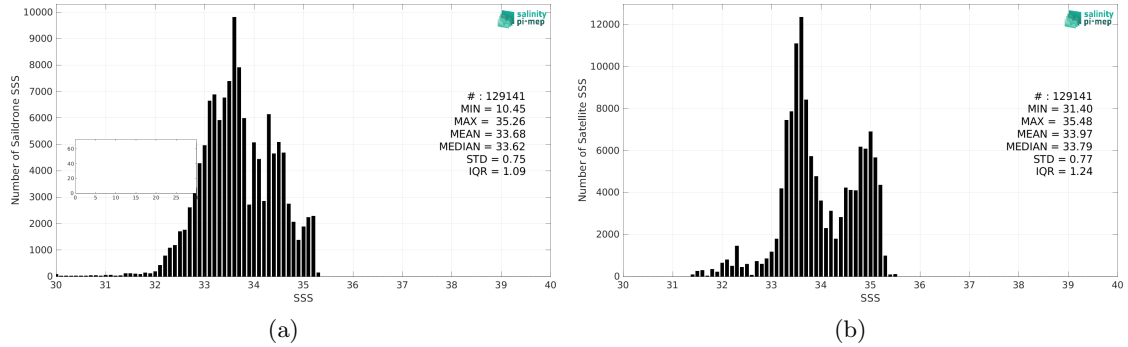
Figure 2: Histograms of SSS from Saildrone (a) and SMOS and SMAP SSS L4 OI v1 - 7 Days (LOPS) (b) considering all match-up pairs per bins of 0.1 over the Mid-Low Latitudes 45N-45S Pi-MEP region and for the full satellite product period.
