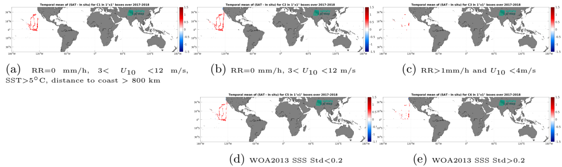
Figure 12: Temporal mean gridded over spatial boxes of size 1^\circ \times 1^\circ of \Delta SSS (SMOS and SMAP SSS L4 OI v1 - 7 Days (LOPS) - Sairdron) for 5 different subdatasets corresponding to: RR=0 mm/h, 3 < U_{10} < 12 m/s, SST > 5^\circ C , distance to coast > 800 km (a), RR=0 mm/h, 3 < U_{10} < 12 m/s (b), RR > 1 mm/h and U_{10} < 4 m/s (c), WOA2013 SSS Std < 0.2 (d), WOA2013 SSS Std > 0.2 (e).
