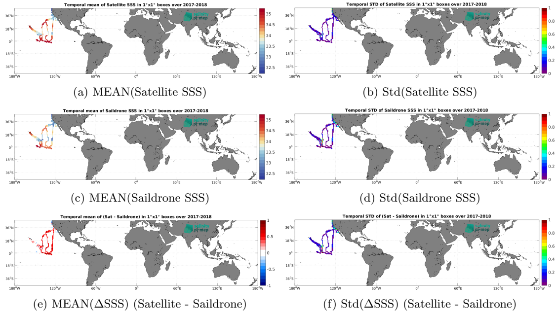
Figure 6: Temporal mean (left) and Std (right) of SSS from SMOS and SMAP SSS L4 OI v1 - 7 Days (LOPS) (top), Saildrone (middle), and of \Delta SSS (Satellite - Saildrone). Only match-up pairs are used to generate these maps.
