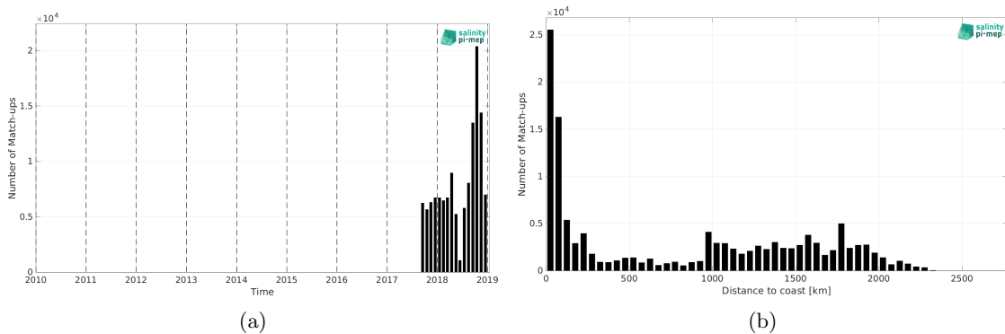
Figure 1: Number of match-ups between Saildrone and SMOS and SMAP SSS L4 OI v1 - 7 Days (LOPS) SSS as a function of time (a) and as function of the distance to coast (b) over the Mid-Low Latitudes 45N-45S Pi-MEP region and for the full satellite product period.
