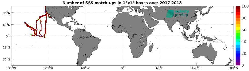
Figure 4: Number of SSS match-ups between Saildrone SSS and the SMOS and SMAP SSS L4 OI v1 - 7 Days (LOPS) SSS product for the Mid-Low Latitudes 45N-45S Pi-MEP region over 1^\circ \times 1^\circ boxes and for the full satellite product period.
