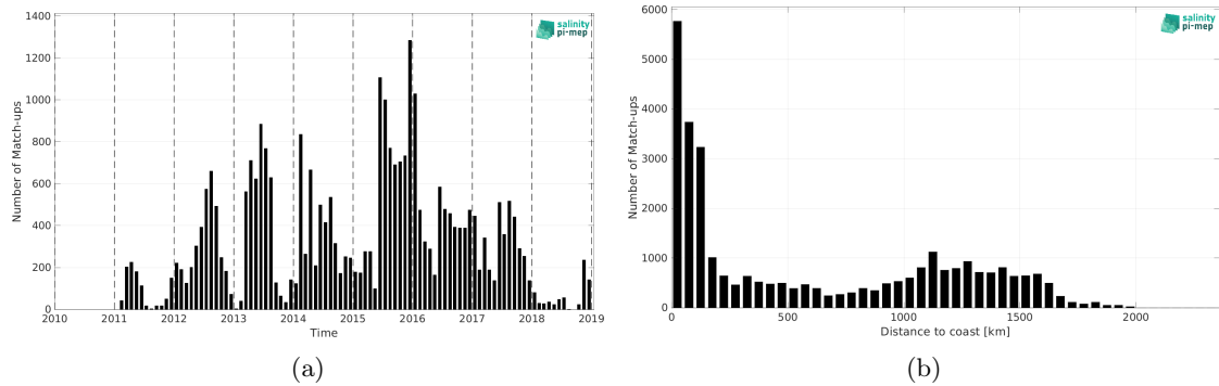
Figure 1: Number of match-ups between Marine mammals and SMOS and SMAP SSS L4 OI v1 - 7 Days (LOPS) SSS as a function of time (a) and as function of the distance to coast (b) over the Mid-Low Latitudes 45N-45S Pi-MEP region and for the full satellite product period.
