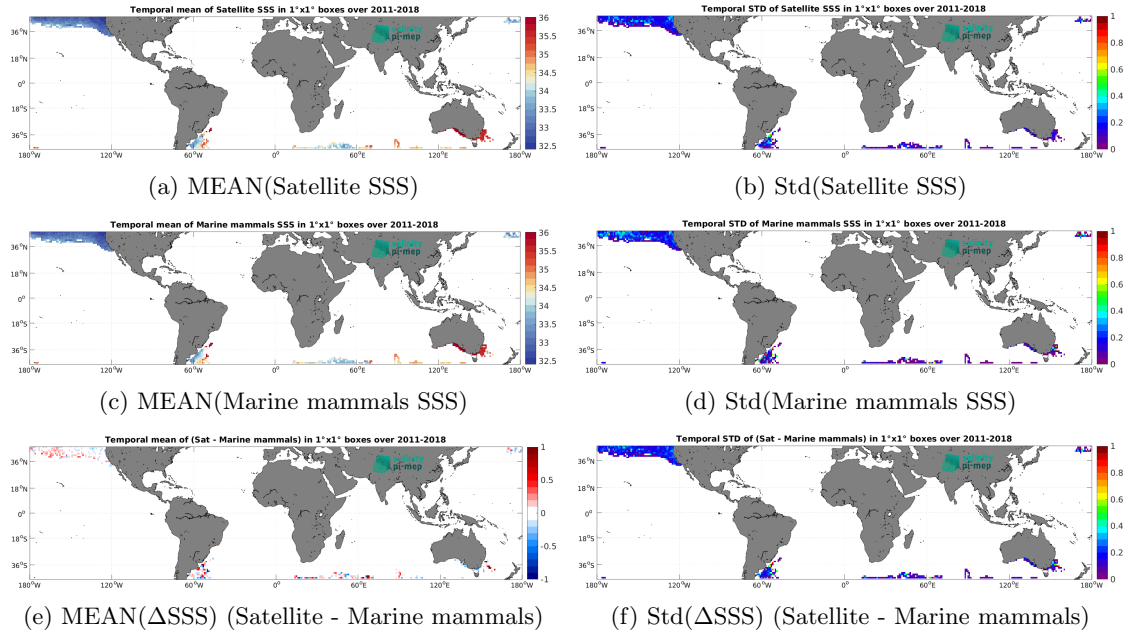
Figure 6: Temporal mean (left) and Std (right) of SSS from SMOS and SMAP SSS L4 OI v1 - 7 Days (LOPS) (top), Marine mammals (middle), and of \Delta SSS (Satellite - Marine mammals). Only match-up pairs are used to generate these maps.
