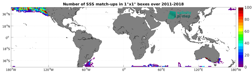
Figure 4: Number of SSS match-ups between Marine mammals SSS and the SMOS and SMAP SSS L4 OI v1 - 7 Days (LOPS) SSS product for the Mid-Low Latitudes 45N-45S Pi-MEP region over 1^\circ \times 1^\circ boxes and for the full satellite product period.
