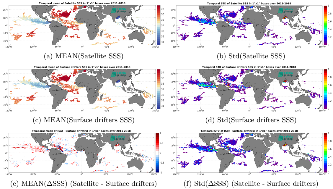
Figure 5: Temporal mean (left) and Std (right) of SSS from SMOS and SMAP SSS L4 OI v1 - 7 Days (LOPS) (top), Surface drifters (middle), and of \Delta SSS (Satellite - Surface drifters). Only match-up pairs are used to generate these maps.
