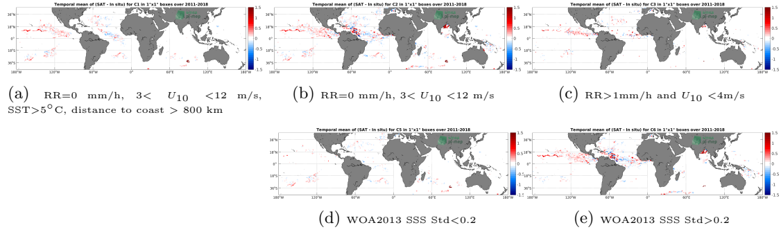
Figure 11: Temporal mean gridded over spatial boxes of size 1^\circ \times 1^\circ of \Delta SSS (SMOS and SMAP SSS L4 OI v1 - 7 Days (LOPS) - Surface drifters) for 5 different subdatasets corresponding to: RR=0 mm/h, 3 < U_{10} < 12 m/s, SST > 5^\circ C , distance to coast > 800 km (a), RR=0 mm/h, 3 < U_{10} < 12 m/s (b), RR > 1 mm/h and U_{10} < 4 m/s (c), WOA2013 SSS Std < 0.2 (d), WOA2013 SSS Std > 0.2 (e).
