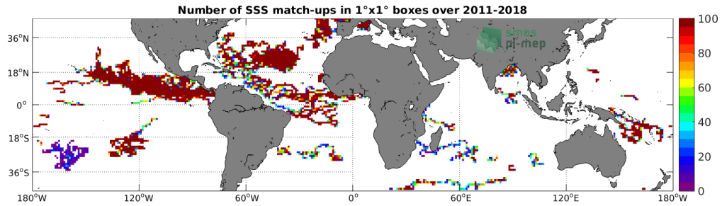
Figure 3: Number of SSS match-ups between Surface drifters SSS and the SMOS and SMAP SSS L4 OI v1 - 7 Days (LOPS) SSS product for the Mid-Low Latitudes 45N-45S Pi-MEP region over 1^\circ \times 1^\circ boxes and for the full satellite product period.
