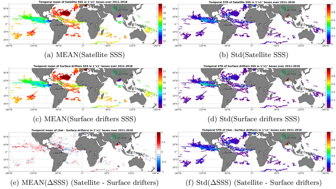
Figure 5: Temporal mean (left) and Std (right) of SSS from SMOS and SMAP SSS L4 OI v1 - 7 Days (LOPS) (top), Surface drifters (middle), and of \Delta SSS (Satellite - Surface drifters). Only match-up pairs are used to generate these maps.
