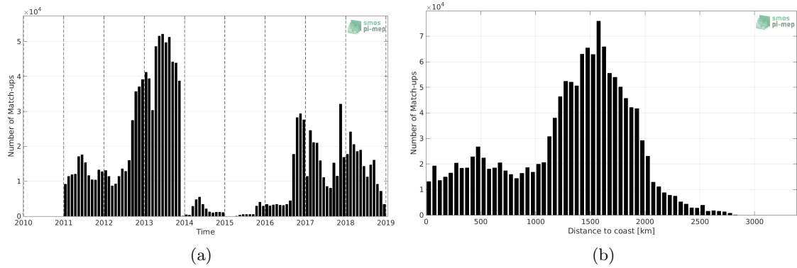
Figure 1: Number of match-ups between Surface drifters and SMOS and SMAP SSS L4 OI v1 - 7 Days (LOPS) SSS as a function of time (a) and as function of the distance to coast (b) over the Mid-Low Latitudes 45N-45S Pi-MEP region and for the full satellite product period.
