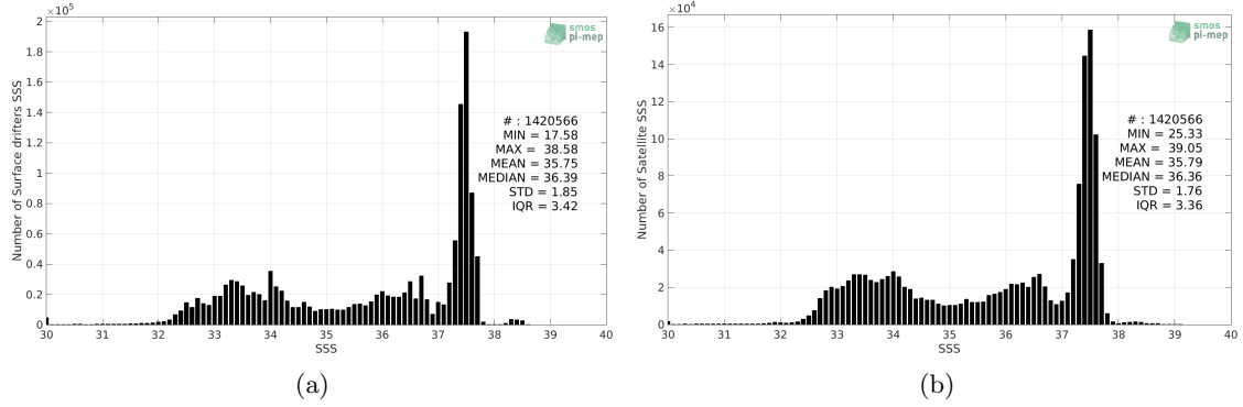
Figure 2: Histograms of SSS from Surface drifters (a) and SMOS and SMAP SSS L4 OI v1 - 7 Days (LOPS) (b) considering all match-up pairs per bins of 0.1 over the Mid-Low Latitudes 45N-45S Pi-MEP region and for the full satellite product period.
