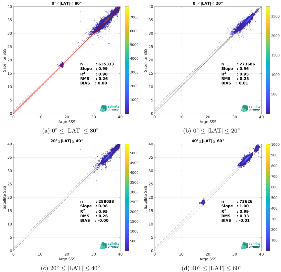
Figure 9: Contour maps of the concentration of SMOS and SMAP SSS L4 OI v1 - 7 Days (LOPS) SSS (y-axis) versus Argo SSS (x-axis) at match-up pairs for different latitude bands. For each plot, the red line shows x=y . The black thin and dashed lines indicate a linear fit through the data cloud and the \pm 95\% confidence levels, respectively. The number match-up pairs n , the slope and R^2 coefficient of the linear fit, the root mean square (RMS) and the mean bias between satellite and in situ data are indicated for each latitude band in each plot.
