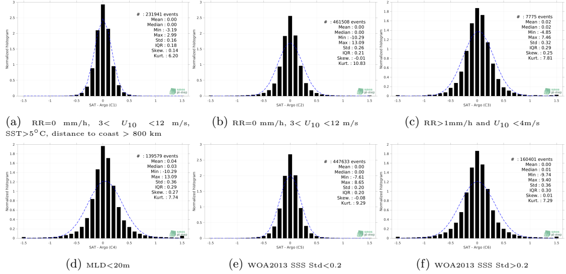
Figure 13: Normalized histogram of \Delta\text{SSS} (SMOS and SMAP SSS L4 OI v1 - 7 Days (LOPS) - Argo) for 6 different subdatasets corresponding to: RR=0 mm/h, 3 < U_{10} < 12 m/s, SST>5°C, distance to coast > 800 km (a), RR=0 mm/h, 3 < U_{10} < 12 m/s (b), RR>1mm/h and U_{10} < 4 m/s (c), MLD<20m (d), WOA2013 SSS Std<0.2 (e), WOA2013 SSS Std>0.2 (f).
