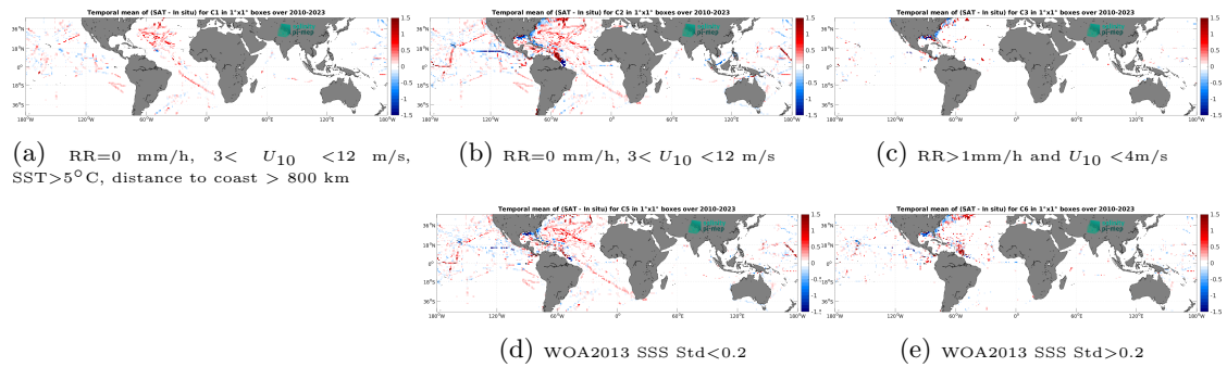
Figure 12: Temporal mean gridded over spatial boxes of size 1^\circ \times 1^\circ of \Delta SSS (SMOS SSS L4 v1 - Weekly (CMEMS-CNR) - TSG (SAMOS)) for 5 different subdatasets corresponding to: RR=0 mm/h, 3 < U_{10} < 12 m/s, SST > 5^\circ\text{C} , distance to coast > 800 km (a), RR=0 mm/h, 3 < U_{10} < 12 m/s (b), RR > 1 mm/h and U_{10} < 4 m/s (c), WOA2013 SSS Std < 0.2 (d), WOA2013 SSS Std > 0.2 (e).
