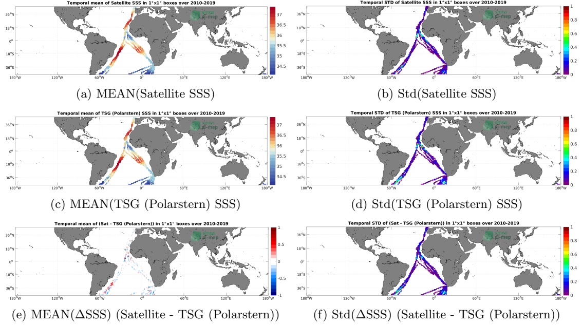
Figure 6: Temporal mean (left) and Std (right) of SSS from SMOS SSS L4 v1 - Weekly (CMEMS-CNR) (top), TSG (Polarstern) (middle), and of \Delta SSS (Satellite - TSG (Polarstern)). Only match-up pairs are used to generate these maps.
