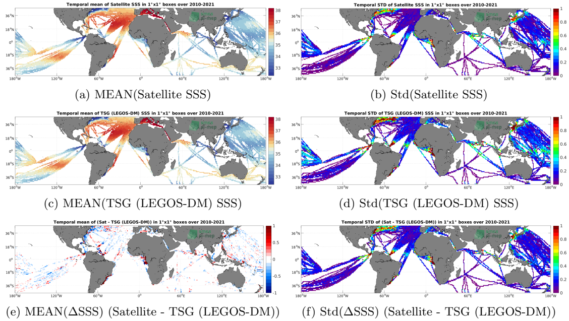
Figure 6: Temporal mean (left) and Std (right) of SSS from SMOS SSS L4 v1 - Weekly (CMEMS-CNR) (top), TSG (LEGOS-DM) (middle), and of \Delta SSS (Satellite - TSG (LEGOS-DM)). Only match-up pairs are used to generate these maps.
