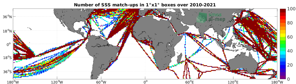
Figure 4: Number of SSS match-ups between TSG (LEGOS-DM) SSS and the SMOS SSS L4 v1 - Weekly (CMEMS-CNR) SSS product for the Mid-Low Latitudes 45N-45S Pi-MEP region over 1^\circ \times 1^\circ boxes and for the full satellite product period.
