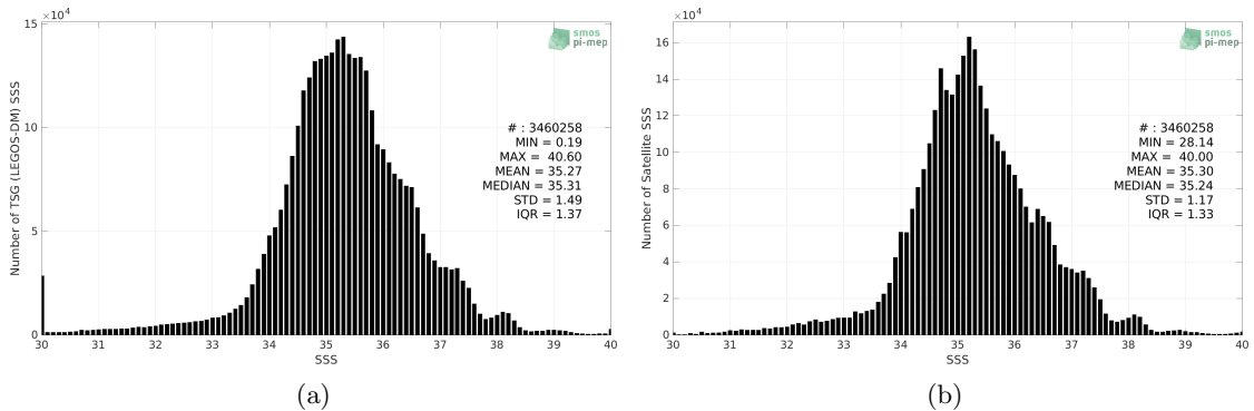
Figure 2: Histograms of SSS from TSG (LEGOS-DM) (a) and SMOS SSS L4 v1 - Weekly (CMEMS-CNR) (b) considering all match-up pairs per bins of 0.1 over the Mid-Low Latitudes 45N-45S Pi-MEP region and for the full satellite product period.
