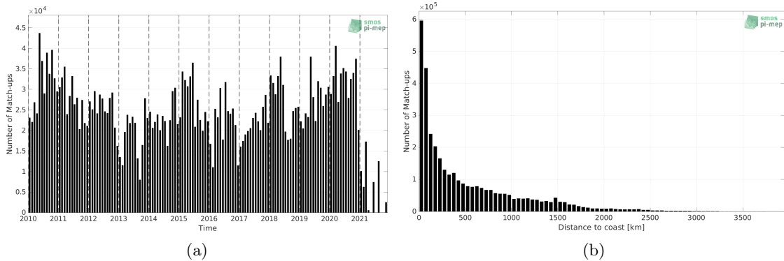
Figure 1: Number of match-ups between TSG (LEGOS-DM) and SMOS SSS L4 v1 - Weekly (CMEMS-CNR) SSS as a function of time (a) and as function of the distance to coast (b) over the Mid-Low Latitudes 45N-45S Pi-MEP region and for the full satellite product period.
