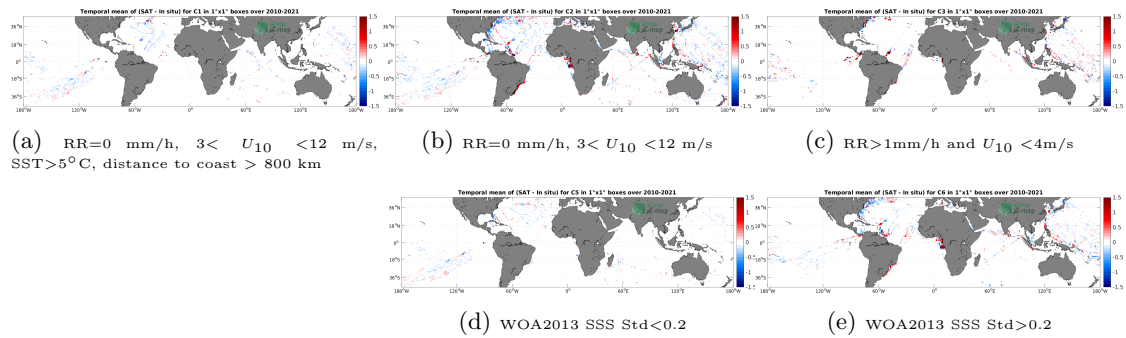
Figure 12: Temporal mean gridded over spatial boxes of size 1^\circ \times 1^\circ of \Delta SSS (SMOS SSS L4 v1 - Weekly (CMEMS-CNR) - TSG (LEGOS-DM)) for 5 different subdatasets corresponding to:RR=0 mm/h, 3 < U_{10} < 12 m/s, SST >5^\circ C, distance to coast > 800 km (a), RR=0 mm/h, 3 < U_{10} < 12 m/s (b), RR >1 mm/h and U_{10} < 4 m/s (c), WOA2013 SSS Std <0.2 (d), WOA2013 SSS Std >0.2 (e).
