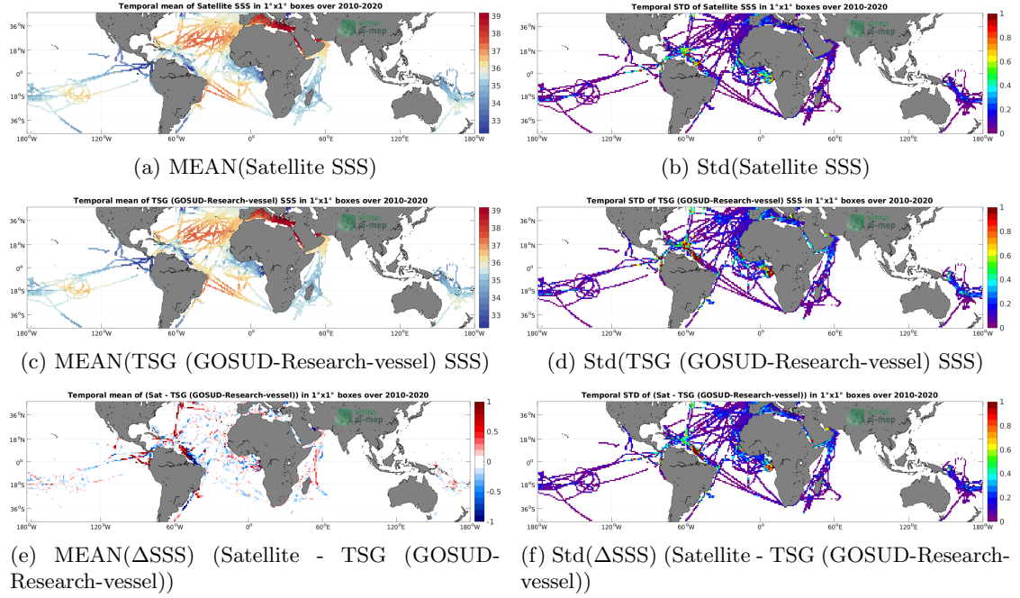
Figure 6: Temporal mean (left) and Std (right) of SSS from SMOS SSS L4 v1 - Weekly (CMEMS-CNR) (top), TSG (GOSUD-Research-vessel) (middle), and of \Delta SSS (Satellite - TSG (GOSUD-Research-vessel)). Only match-up pairs are used to generate these maps.
