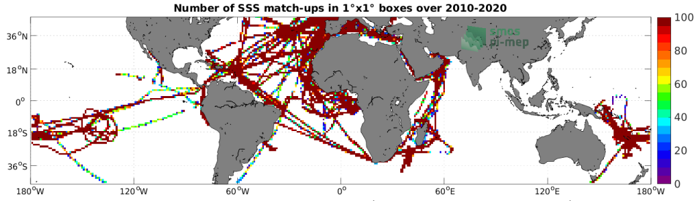
Figure 4: Number of SSS match-ups between TSG (GOSUD-Research-vessel) SSS and the SMOS SSS L4 v1 - Weekly (CMEMS-CNR) SSS product for the Mid-Low Latitudes 45N-45S Pi-MEP region over 1^\circ \times 1^\circ boxes and for the full satellite product period.
