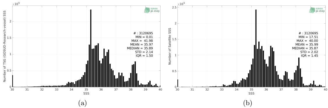
Figure 2: Histograms of SSS from TSG (GOSUD-Research-vessel) (a) and SMOS SSS L4 v1 - Weekly (CMEMS-CNR) (b) considering all match-up pairs per bins of 0.1 over the Mid-Low Latitudes 45N-45S Pi-MEP region and for the full satellite product period.
