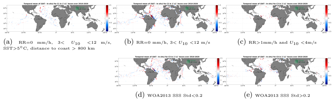
Figure 12: Temporal mean gridded over spatial boxes of size 1^\circ \times 1^\circ of \Delta SSS (SMOS SSS L4 v1 - Weekly (CMEMS-CNR) - TSG (GOSUD-Research-vessel)) for 5 different subdatasets corresponding to:RR=0 mm/h, 3 < U_{10} < 12 m/s, SST >5^\circ C, distance to coast > 800 km (a), RR=0 mm/h, 3 < U_{10} < 12 m/s (b), RR >1 mm/h and U_{10} < 4 m/s (c), WOA2013 SSS Std <0.2 (d), WOA2013 SSS Std >0.2 (e).
