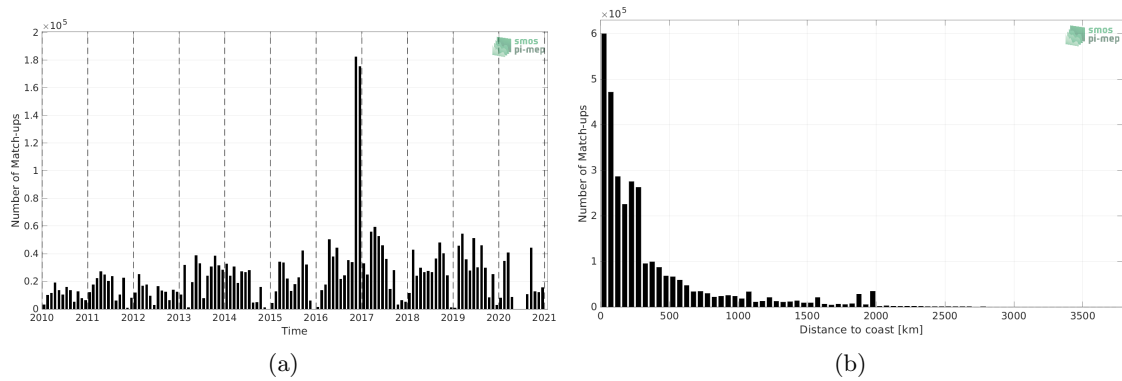
Figure 1: Number of match-ups between TSG (GOSUD-Research-vessel) and SMOS SSS L4 v1 - Weekly (CMEMS-CNR) SSS as a function of time (a) and as function of the distance to coast (b) over the Mid-Low Latitudes 45N-45S Pi-MEP region and for the full satellite product period.
