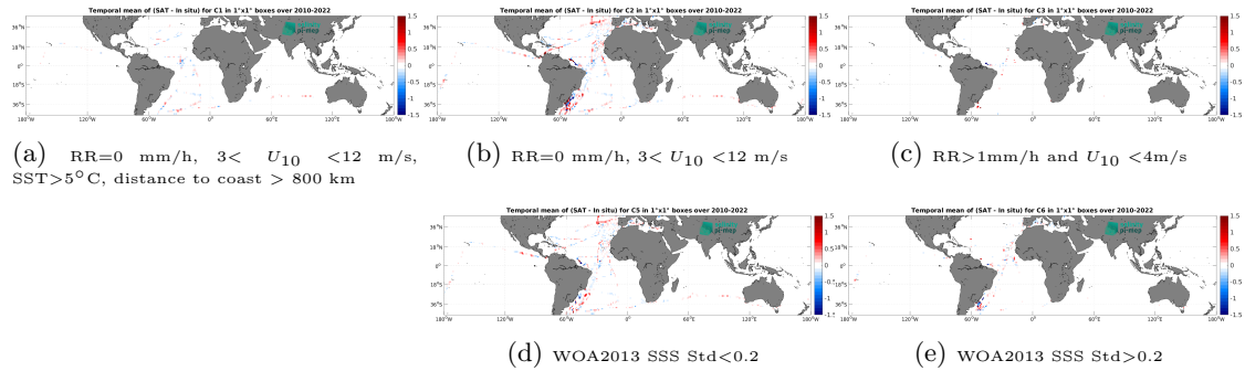
Figure 12: Temporal mean gridded over spatial boxes of size 1^\circ \times 1^\circ of \Delta SSS (SMOS SSS L4 v1 - Weekly (CMEMS-CNR) - TSG (CSIC-UTM)) for 5 different subdatasets corresponding to: RR=0 mm/h, 3 < U_{10} < 12 m/s, SST > 5^\circ\text{C} , distance to coast > 800 km (a), RR=0 mm/h, 3 < U_{10} < 12 m/s (b), RR > 1\text{mm/h} and U_{10} < 4\text{m/s} (c), WOA2013 SSS Std < 0.2 (d), WOA2013 SSS Std > 0.2 (e).
