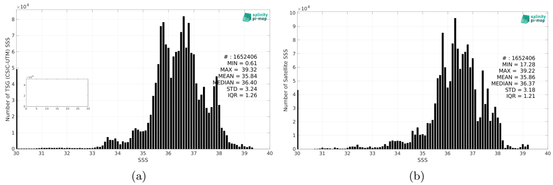
Figure 2: Histograms of SSS from TSG (CSIC-UTM) (a) and SMOS SSS L4 v1 - Weekly (CMEMS-CNR) (b) considering all match-up pairs per bins of 0.1 over the Mid-Low Latitudes 45N-45S Pi-MEP region and for the full satellite product period.
