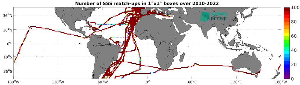
Figure 4: Number of SSS match-ups between TSG (CSIC-UTM) SSS and the SMOS SSS L4 v1 - Weekly (CMEMS-CNR) SSS product for the Mid-Low Latitudes 45N-45S Pi-MEP region over 1^\circ \times 1^\circ boxes and for the full satellite product period.
