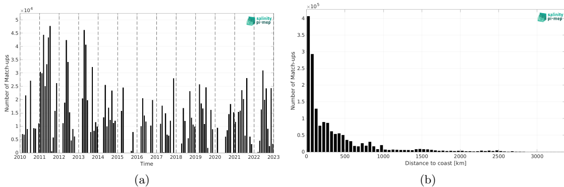
Figure 1: Number of match-ups between TSG (CSIC-UTM) and SMOS SSS L4 v1 - Weekly (CMEMS-CNR) SSS as a function of time (a) and as function of the distance to coast (b) over the Mid-Low Latitudes 45N-45S Pi-MEP region and for the full satellite product period.
