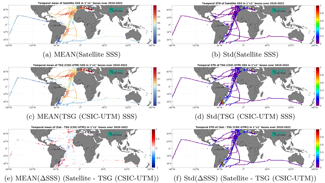
Figure 6: Temporal mean (left) and Std (right) of SSS from SMOS SSS L4 v1 - Weekly (CMEMS-CNR) (top), TSG (CSIC-UTM) (middle), and of \Delta SSS (Satellite - TSG (CSIC-UTM)). Only match-up pairs are used to generate these maps.
