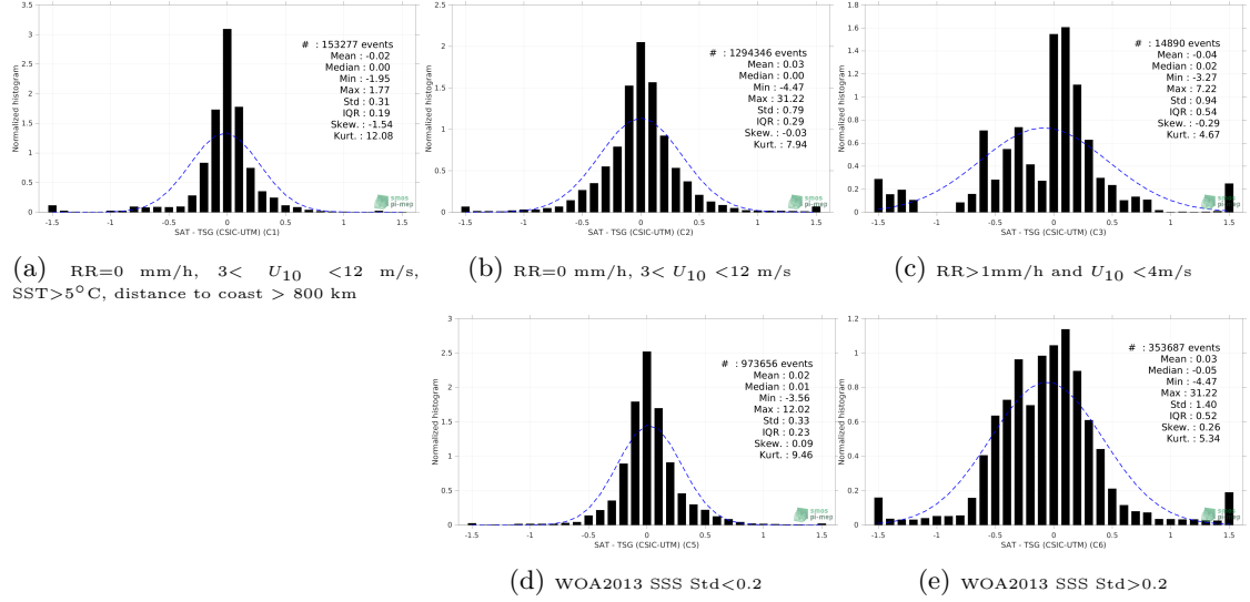
Figure 13: Normalized histogram of \Delta SSS (SMOS SSS L4 v1 - Weekly (CMEMS-CNR) - TSG (CSIC-UTM)) for 5 different subdatasets corresponding to: RR=0 mm/h, 3 < U_{10} < 12 m/s, SST > 5°C, distance to coast > 800 km (a), RR=0 mm/h, 3 < U_{10} < 12 m/s (b), RR > 1mm/h and U_{10} < 4 m/s (c), WOA2013 SSS Std < 0.2 (d), WOA2013 SSS Std > 0.2 (e).
