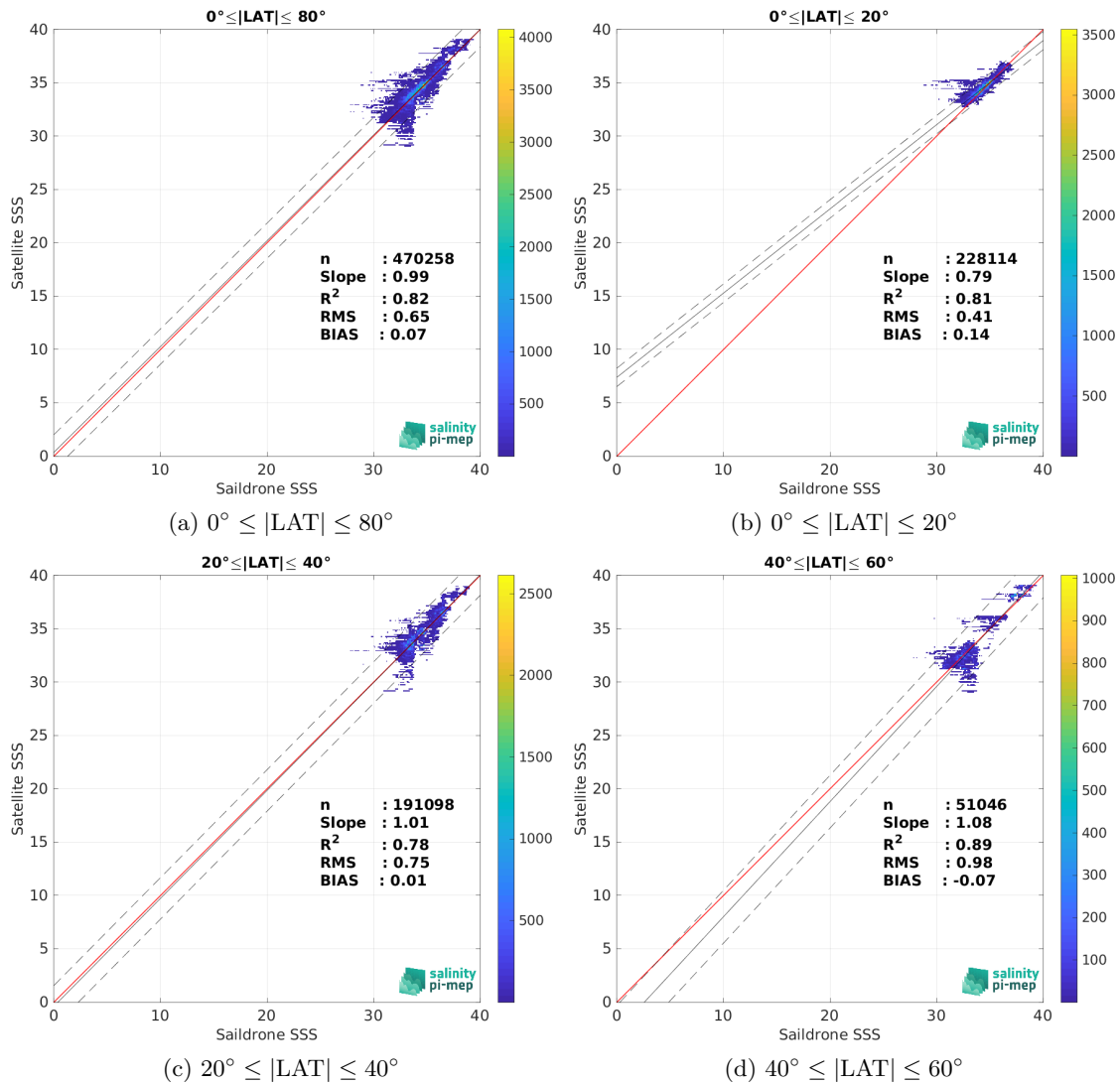
Figure 9: Contour maps of the concentration of SMOS SSS L4 v1 - Weekly (CMEMS-CNR) SSS (y-axis) versus Sairdrone SSS (x-axis) at match-up pairs for different latitude bands. For each plot, the red line shows x=y . The black thin and dashed lines indicate a linear fit through the data cloud and the \pm 95\% confidence levels, respectively. The number match-up pairs n , the slope and R^2 coefficient of the linear fit, the root mean square (RMS) and the mean bias between satellite and in situ data are indicated for each latitude band in each plots.
