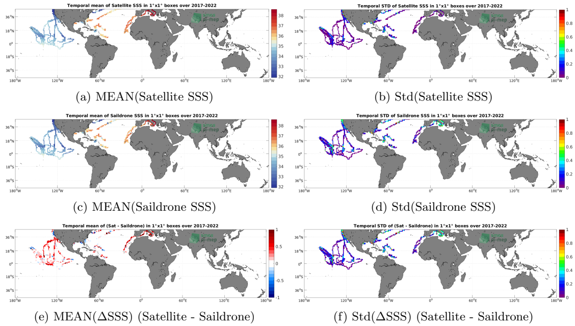
Figure 6: Temporal mean (left) and Std (right) of SSS from SMOS SSS L4 v1 - Weekly (CMEMS-CNR) (top), Saildrone (middle), and of \Delta SSS (Satellite - Saildrone). Only match-up pairs are used to generate these maps.
