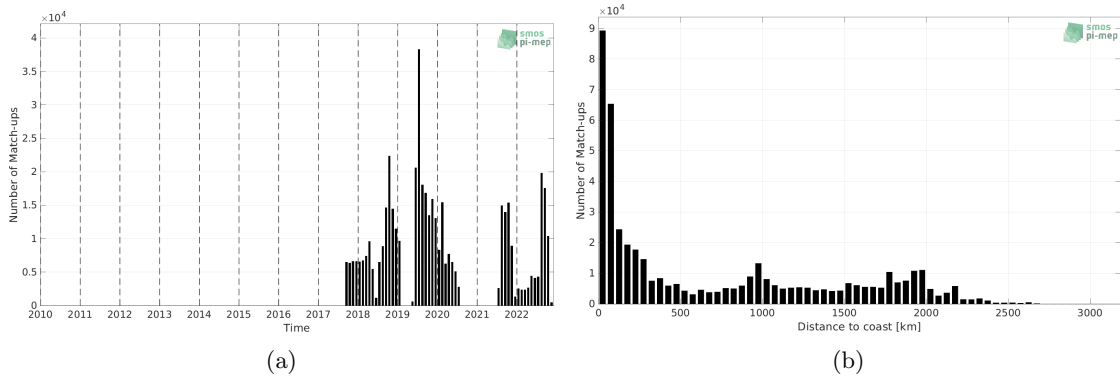
Figure 1: Number of match-ups between Saildrone and SMOS SSS L4 v1 - Weekly (CMEMS-CNR) SSS as a function of time (a) and as function of the distance to coast (b) over the Mid-Low Latitudes 45N-45S Pi-MEP region and for the full satellite product period.
