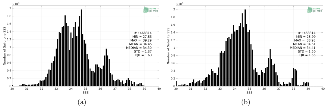
Figure 2: Histograms of SSS from Saildrone (a) and SMOS SSS L4 v1 - Weekly (CMEMS-CNR) (b) considering all match-up pairs per bins of 0.1 over the Mid-Low Latitudes 45N-45S Pi-MEP region and for the full satellite product period.
