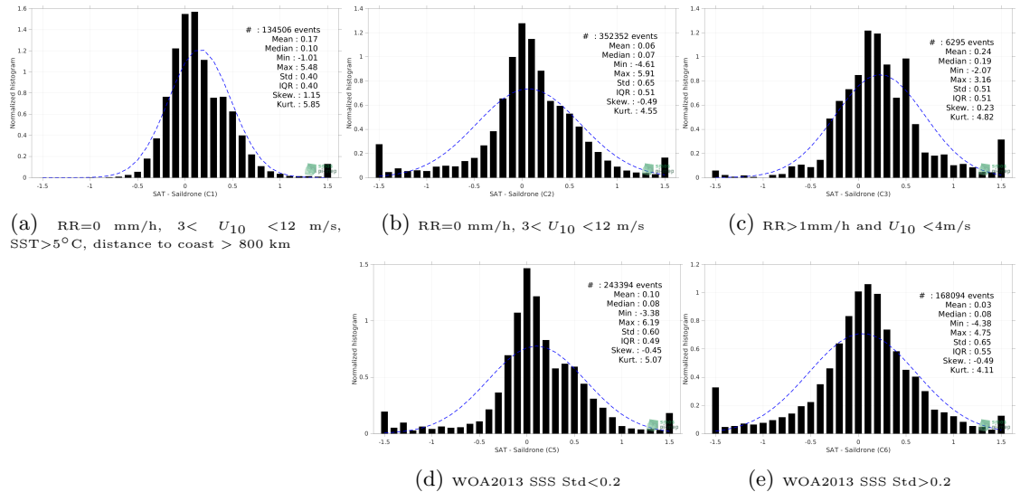
Figure 13: Normalized histogram of \Delta SSS (SMOS SSS L4 v1 - Weekly (CMEMS-CNR) - Saildrone) for 5 different subdatasets corresponding to: RR=0 mm/h, 3 < U_{10} < 12 m/s, SST >5^\circ\text{C} , distance to coast > 800 km (a), RR=0 mm/h, 3 < U_{10} < 12 m/s (b), RR >1 mm/h and U_{10} < 4 m/s (c), WOA2013 SSS Std <0.2 (d), WOA2013 SSS Std >0.2 (e).
