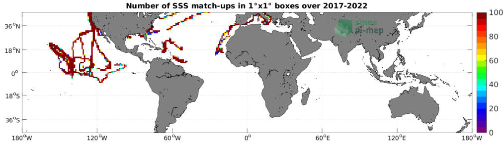
Figure 4: Number of SSS match-ups between Saildrone SSS and the SMOS SSS L4 v1 - Weekly (CMEMS-CNR) SSS product for the Mid-Low Latitudes 45N-45S Pi-MEP region over 1^\circ \times 1^\circ boxes and for the full satellite product period.
