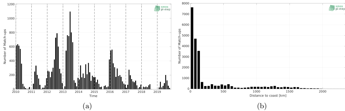
Figure 1: Number of match-ups between Marine mammals and SMOS SSS L4 v1 - Weekly (CMEMS-CNR) SSS as a function of time (a) and as function of the distance to coast (b) over the Mid-Low Latitudes 45N-45S Pi-MEP region and for the full satellite product period.
