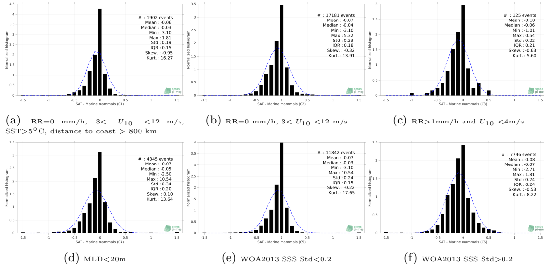
Figure 13: Normalized histogram of \Delta SSS (SMOS SSS L4 v1 - Weekly (CMEMS-CNR) - Marine mammals) for 6 different subdatasets corresponding to: RR=0 mm/h, 3 < U_{10} < 12 m/s, SST > 5°C, distance to coast > 800 km (a), RR=0 mm/h, 3 < U_{10} < 12 m/s (b), RR > 1mm/h and U_{10} < 4 m/s (c), MLD < 20m (d), WOA2013 SSS Std < 0.2 (e), WOA2013 SSS Std > 0.2 (f).
