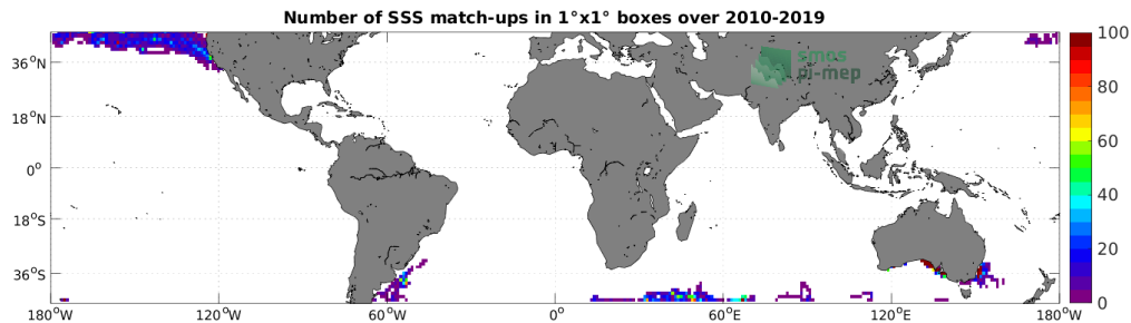
Figure 4: Number of SSS match-ups between Marine mammals SSS and the SMOS SSS L4 v1 - Weekly (CMEMS-CNR) SSS product for the Mid-Low Latitudes 45N-45S Pi-MEP region over 1^\circ \times 1^\circ boxes and for the full satellite product period.
