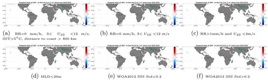
Figure 12: Temporal mean gridded over spatial boxes of size 1^\circ \times 1^\circ of \Delta SSS (SMOS SSS L4 v1 - Weekly (CMEMS-CNR) - Marine mammals) for 6 different subdatasets corresponding to:RR=0 mm/h, 3 < U_{10} < 12 m/s, SST >5^\circ C, distance to coast > 800 km (a), RR=0 mm/h, 3 < U_{10} < 12 m/s (b), RR >1 mm/h and U_{10} < 4 m/s (c),MLD <20 m (d),WOA2013 SSS Std <0.2 (e),WOA2013 SSS Std >0.2 (f).
