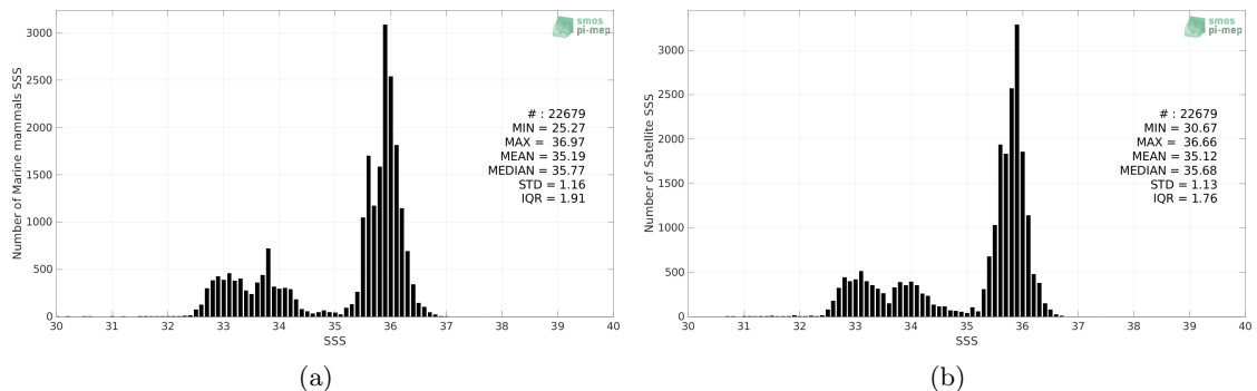
Figure 2: Histograms of SSS from Marine mammals (a) and SMOS SSS L4 v1 - Weekly (CMEMS-CNR) (b) considering all match-up pairs per bins of 0.1 over the Mid-Low Latitudes 45N-45S Pi-MEP region and for the full satellite product period.
