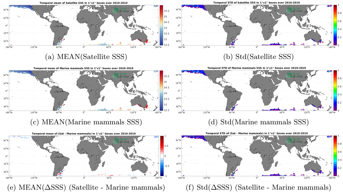
Figure 6: Temporal mean (left) and Std (right) of SSS from SMOS SSS L4 v1 - Weekly (CMEMS-CNR) (top), Marine mammals (middle), and of \Delta SSS (Satellite - Marine mammals). Only match-up pairs are used to generate these maps.
