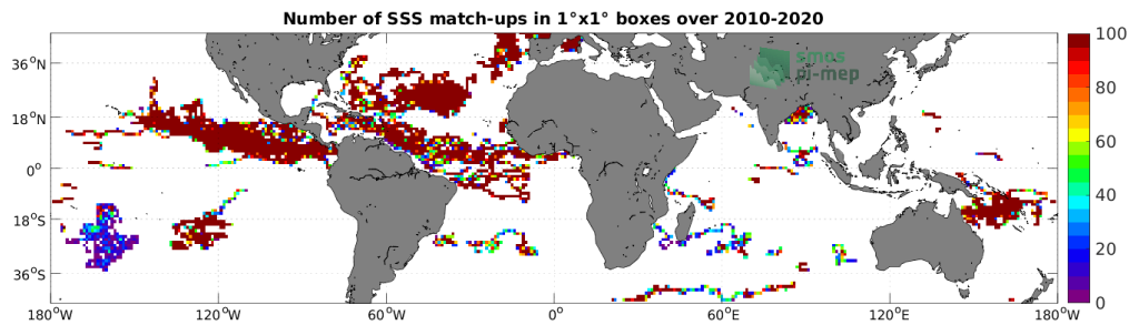
Figure 3: Number of SSS match-ups between Surface drifters SSS and the SMOS SSS L4 v1 - Weekly (CMEMS-CNR) SSS product for the Mid-Low Latitudes 45N-45S Pi-MEP region over 1^\circ \times 1^\circ boxes and for the full satellite product period.
