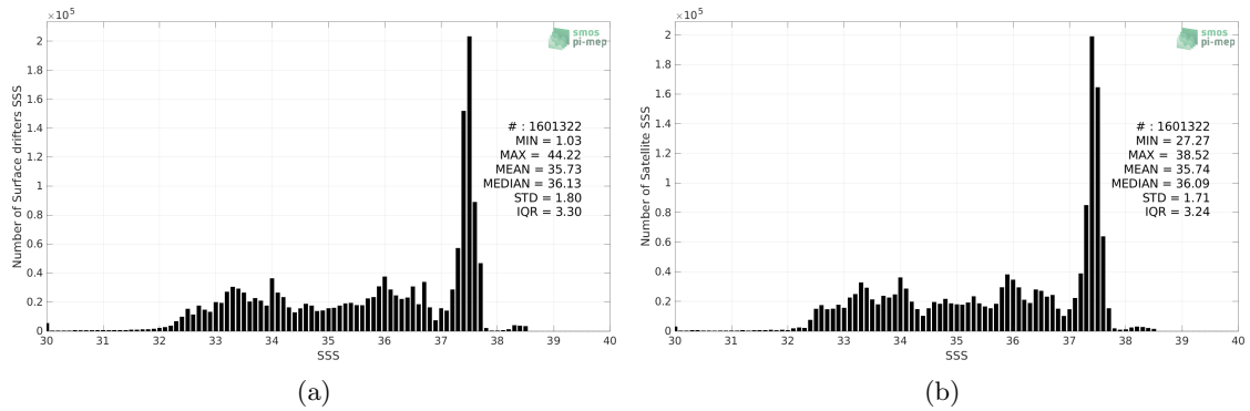
Figure 2: Histograms of SSS from Surface drifters (a) and SMOS SSS L4 v1 - Weekly (CMEMS-CNR) (b) considering all match-up pairs per bins of 0.1 over the Mid-Low Latitudes 45N-45S Pi-MEP region and for the full satellite product period.
