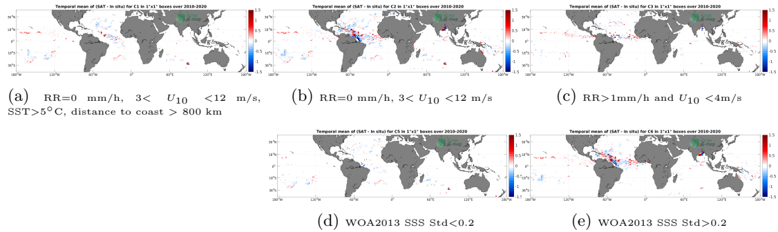
Figure 11: Temporal mean gridded over spatial boxes of size 1^\circ \times 1^\circ of \Delta SSS (SMOS SSS L4 v1 - Weekly (CMEMS-CNR) - Surface drifters) for 5 different subdatasets corresponding to: RR=0 mm/h, 3 < U_{10} < 12 m/s, SST > 5^\circ\text{C} , distance to coast > 800 km (a), RR=0 mm/h, 3 < U_{10} < 12 m/s (b), RR > 1\text{mm/h} and U_{10} < 4\text{m/s} (c), WOA2013 SSS Std < 0.2 (d), WOA2013 SSS Std > 0.2 (e).
