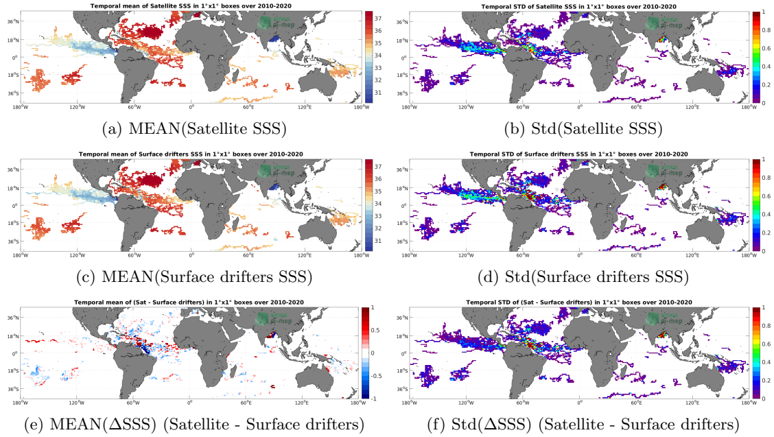
Figure 5: Temporal mean (left) and Std (right) of SSS from SMOS SSS L4 v1 - Weekly (CMEMS-CNR) (top), Surface drifters (middle), and of \Delta SSS (Satellite - Surface drifters). Only match-up pairs are used to generate these maps.
