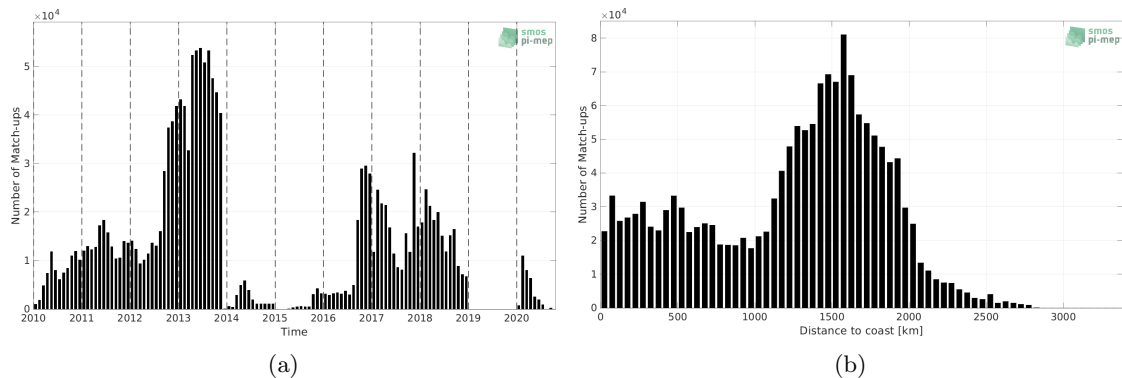
Figure 1: Number of match-ups between Surface drifters and SMOS SSS L4 v1 - Weekly (CMEMS-CNR) SSS as a function of time (a) and as function of the distance to coast (b) over the Mid-Low Latitudes 45N-45S Pi-MEP region and for the full satellite product period.
