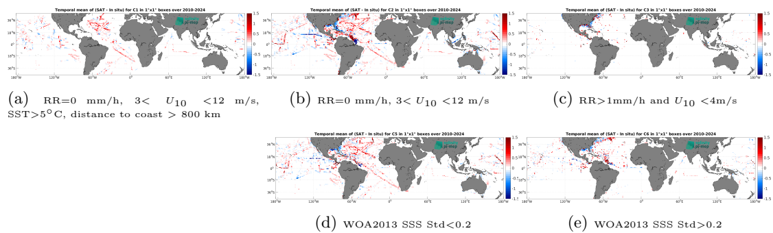
Figure 14: Temporal mean gridded over spatial boxes of size 1^\circ \times 1^\circ of \Delta\text{SSS} (SMOS SSS L4 v1 - Monthly (CMEMS-CNR) - TSG (SAMOS)) for 5 different subdatasets corresponding to: RR=0 mm/h, 3 < U_{10} < 12 m/s, SST > 5°C, distance to coast > 800 km (a), RR=0 mm/h, 3 < U_{10} < 12 m/s (b), RR > 1mm/h and U_{10} < 4 m/s (c), WOA2013 SSS Std < 0.2 (d), WOA2013 SSS Std > 0.2 (e).
