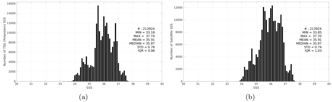
Figure 3: Histograms of SSS from TSG (Polarstern) (a) and SMOS SSS L4 v1 - Monthly (CMEMS-CNR) (b) considering all match-up pairs per bins of 0.1 over the Mid-Low Latitudes 45N-45S Pi-MEP region and for the full satellite product period.
