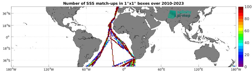
Figure 5: Number of SSS match-ups between TSG (Polarstern) SSS and the SMOS SSS L4 v1 - Monthly (CMEMS-CNR) SSS product for the Mid-Low Latitudes 45N-45S Pi-MEP region over 1^\circ \times 1^\circ boxes and for the full satellite product period.
