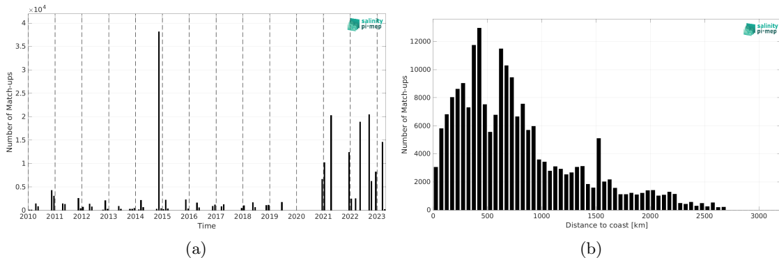
Figure 2: Number of match-ups between TSG (Polarstern) and SMOS SSS L4 v1 - Monthly (CMEMS-CNR) SSS as a function of time (a) and as function of the distance to coast (b) over the Mid-Low Latitudes 45N-45S Pi-MEP region and for the full satellite product period.
