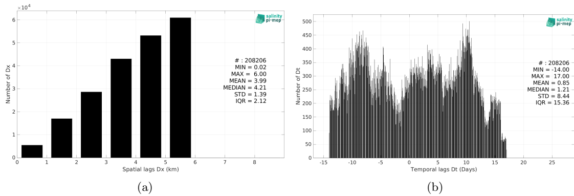
Figure 6: Histograms of the spatial (a) and temporal (b) lags between the location/time of the TSG (Polarstern) measurement and the date of the corresponding SMOS SSS L4 v1 - Monthly (CMEMS-CNR) SSS pixel.
