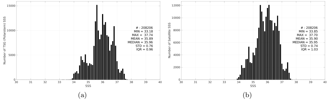
Figure 3: Histograms of SSS from TSG (Polarstern) (a) and SMOS SSS L4 v1 - Monthly (CMEMS-CNR) (b) considering all match-up pairs per bins of 0.1 over the Mid-Low Latitudes 45N-45S Pi-MEP region and for the full satellite product period.
