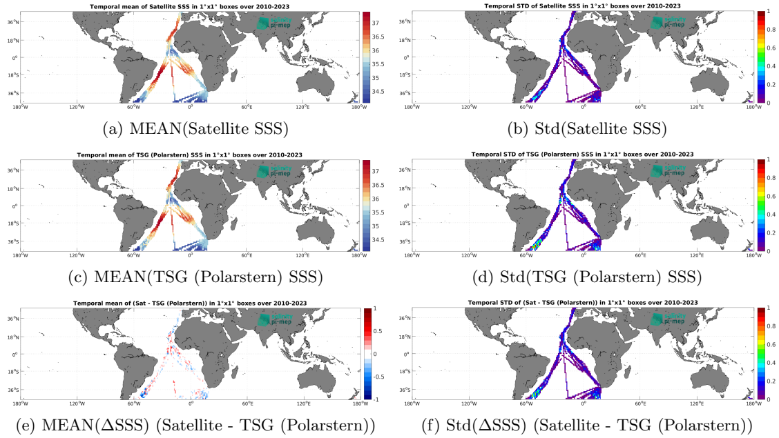
Figure 7: Temporal mean (left) and Std (right) of SSS from SMOS SSS L4 v1 - Monthly (CMEMS-CNR) (top), TSG (Polarstern) (middle), and of \Delta SSS (Satellite - TSG (Polarstern)). Only match-up pairs are used to generate these maps.
