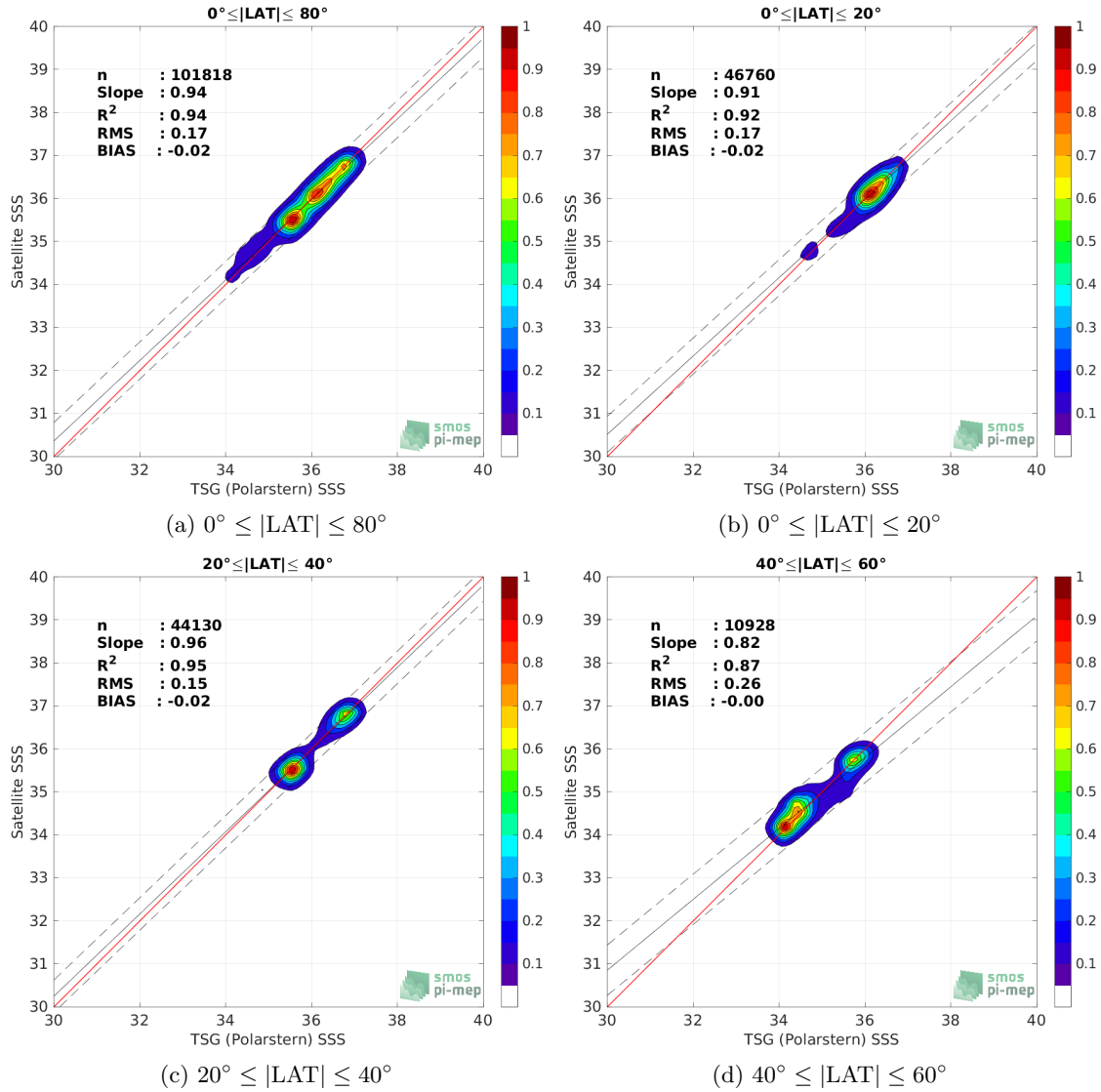
Figure 9: Contour maps of the concentration of SMOS SSS L4 v1 - Monthly (CMEMS-CNR) SSS (y-axis) versus TSG (Polarstern) SSS (x-axis) at match-up pairs for different latitude bands. For each plot, the red line shows x=y . The black thin and dashed lines indicate a linear fit through the data cloud and the \pm 95\% confidence levels, respectively. The number match-up pairs n , the slope and R^2 coefficient of the linear fit, the root mean square (RMS) and the mean bias between satellite and in situ data are indicated for each latitude band in each plots.
