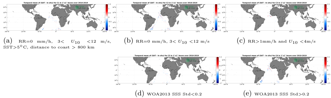
Figure 12: Temporal mean gridded over spatial boxes of size 1^\circ \times 1^\circ of \Delta SSS (SMOS SSS L4 v1 - Monthly (CMEMS-CNR) - TSG (Polarstern)) for 5 different subdatasets corresponding to:RR=0 mm/h, 3 < U_{10} < 12 m/s, SST >5^\circ\text{C} , distance to coast > 800 km (a), RR=0 mm/h, 3 < U_{10} < 12 m/s (b), RR >1 mm/h and U_{10} < 4 m/s (c), WOA2013 SSS Std <0.2 (d), WOA2013 SSS Std >0.2 (e).
