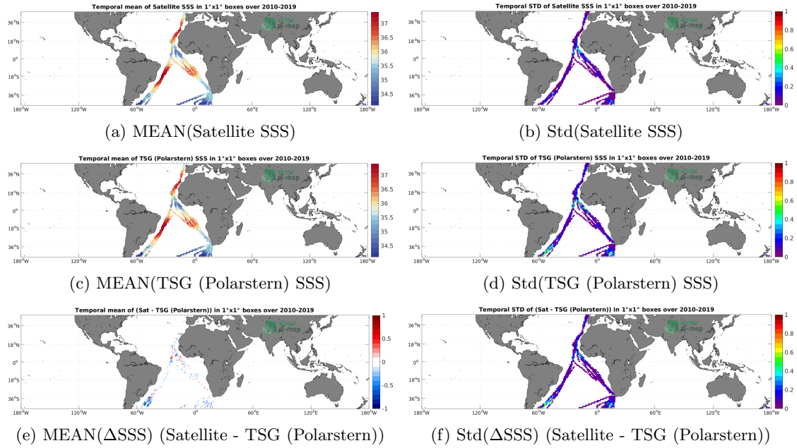
Figure 6: Temporal mean (left) and Std (right) of SSS from SMOS SSS L4 v1 - Monthly (CMEMS-CNR) (top), TSG (Polarstern) (middle), and of \Delta SSS (Satellite - TSG (Polarstern)). Only match-up pairs are used to generate these maps.
