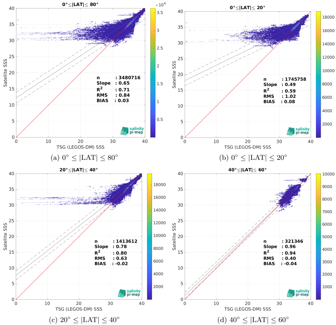
Figure 10: Contour maps of the concentration of SMOS SSS L4 v1 - Monthly (CMEMS-CNR) SSS (y-axis) versus TSG (LEGOS-DM) SSS (x-axis) at match-up pairs for different latitude bands. For each plot, the red line shows x=y . The black thin and dashed lines indicate a linear fit through the data cloud and the \pm 95\% confidence levels, respectively. The number match-up pairs n , the slope and R^2 coefficient of the linear fit, the root mean square (RMS) and the mean bias between satellite and in situ data are indicated for each latitude band in each plots.
