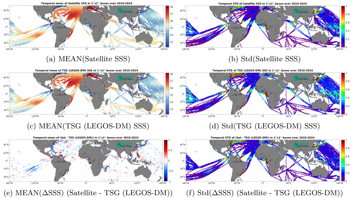
Figure 7: Temporal mean (left) and Std (right) of SSS from SMOS SSS L4 v1 - Monthly (CMEMS-CNR) (top), TSG (LEGOS-DM) (middle), and of \Delta SSS (Satellite - TSG (LEGOS-DM)). Only match-up pairs are used to generate these maps.
