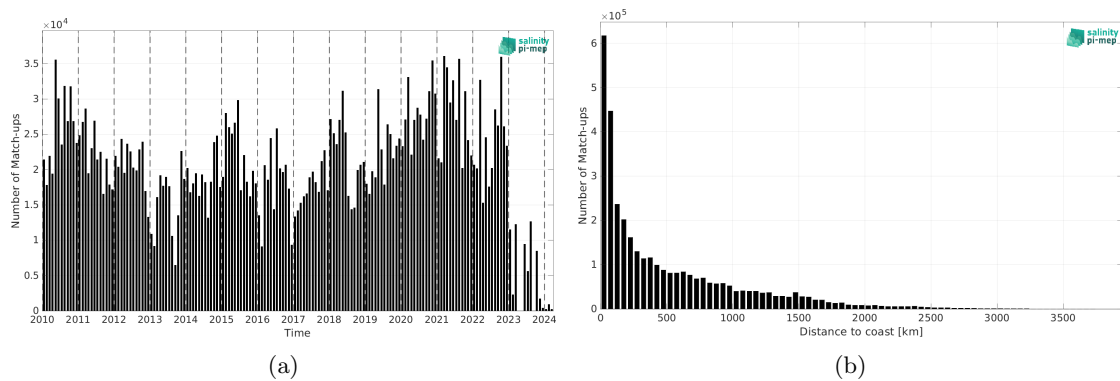
Figure 2: Number of match-ups between TSG (LEGOS-DM) and SMOS SSS L4 v1 - Monthly (CMEMS-CNR) SSS as a function of time (a) and as function of the distance to coast (b) over the Mid-Low Latitudes 45N-45S Pi-MEP region and for the full satellite product period.
