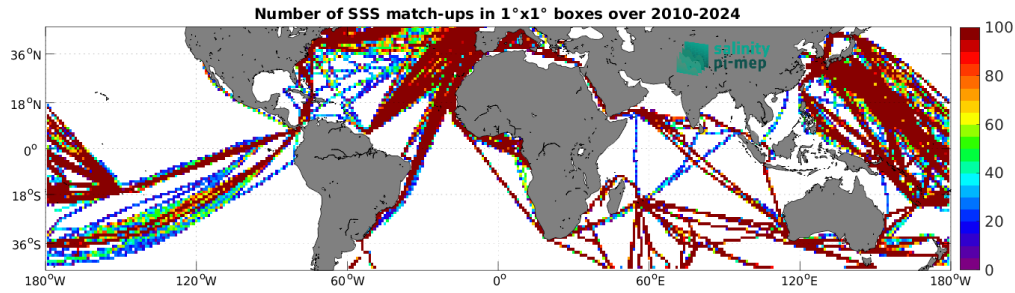
Figure 5: Number of SSS match-ups between TSG (LEGOS-DM) SSS and the SMOS SSS L4 v1 - Monthly (CMEMS-CNR) SSS product for the Mid-Low Latitudes 45N-45S Pi-MEP region over 1^\circ \times 1^\circ boxes and for the full satellite product period.
