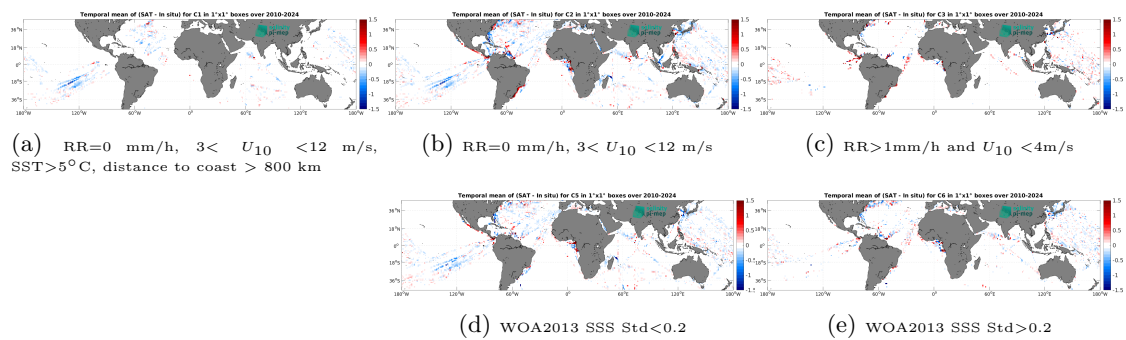
Figure 14: Temporal mean gridded over spatial boxes of size 1^\circ \times 1^\circ of \Delta SSS (SMOS SSS L4 v1 - Monthly (CMEMS-CNR) - TSG (LEGOS-DM)) for 5 different subdatasets corresponding to: RR=0 mm/h, 3 < U_{10} < 12 m/s, SST > 5°C, distance to coast > 800 km (a), RR=0 mm/h, 3 < U_{10} < 12 m/s (b), RR > 1mm/h and U_{10} < 4 m/s (c), WOA2013 SSS Std < 0.2 (d), WOA2013 SSS Std > 0.2 (e).
