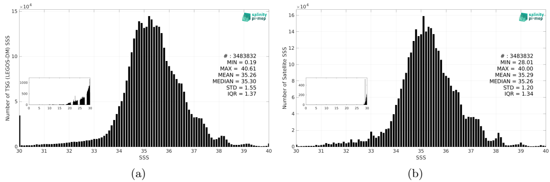
Figure 3: Histograms of SSS from TSG (LEGOS-DM) (a) and SMOS SSS L4 v1 - Monthly (CMEMS-CNR) (b) considering all match-up pairs per bins of 0.1 over the Mid-Low Latitudes 45N-45S Pi-MEP region and for the full satellite product period.
